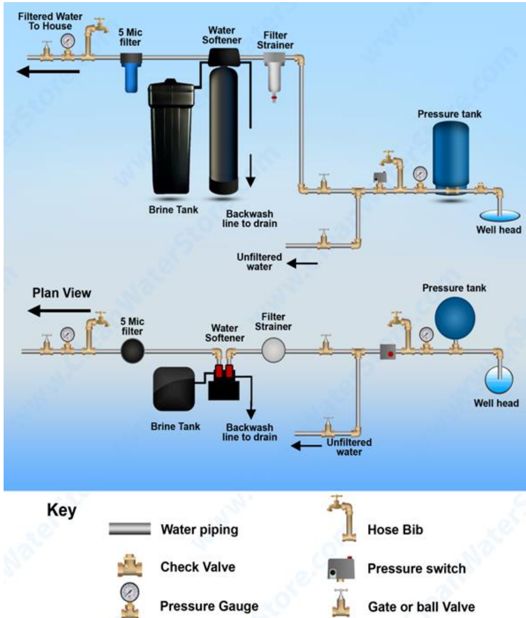
Fig 2 - Typical Softener Fleck 5600-SXT piping installation with ball valve and hose bib after the filter along with pre- and post-filtration if necessary:
