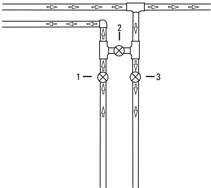
Figure 6 Knob Style Plastic Bypass Valve
