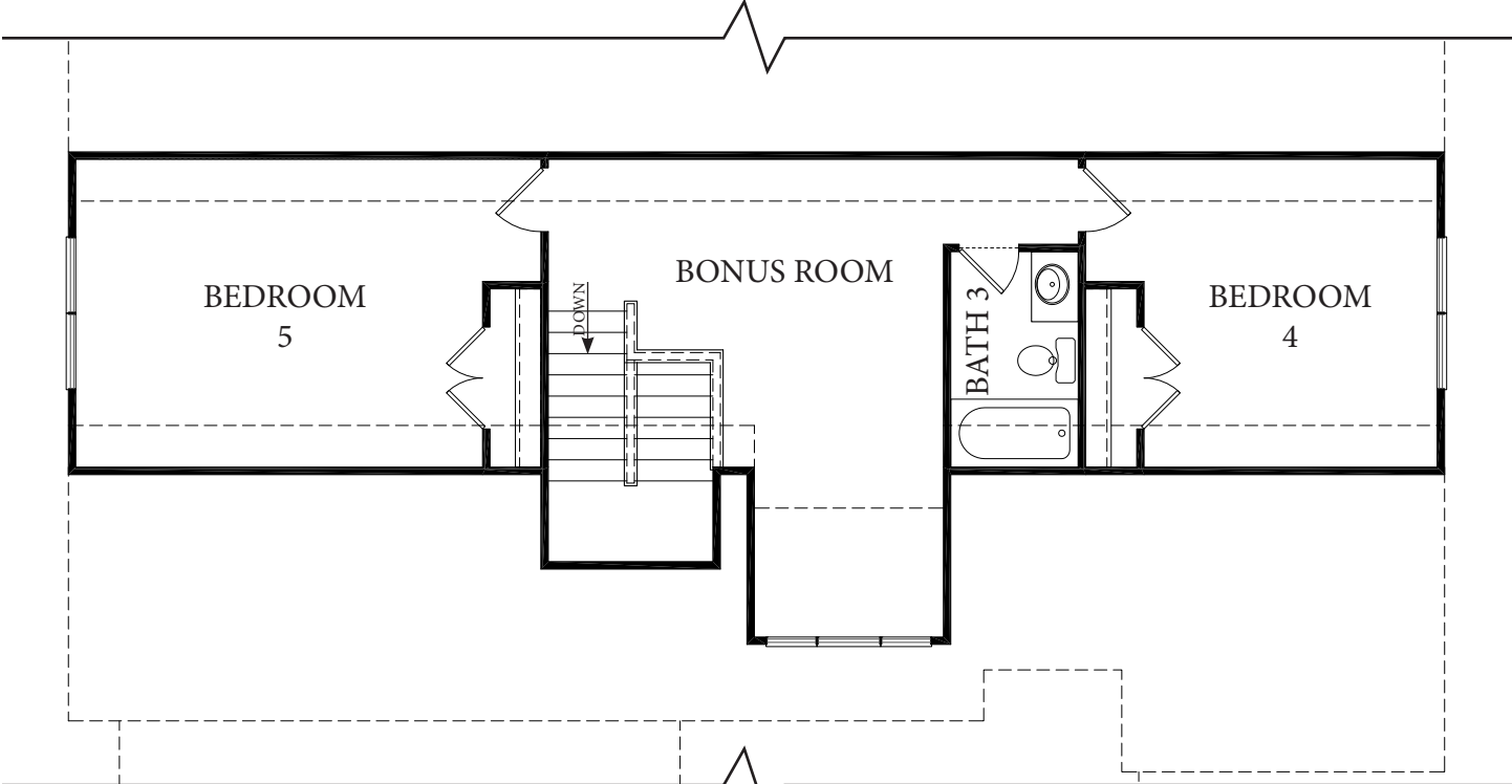
OPT. SECOND FLOOR - BONUS ROOM W/ BEDROOM
