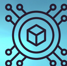
Tokenization
