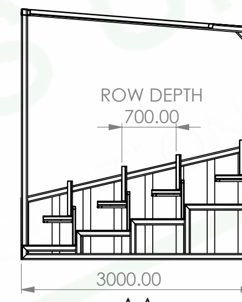
TYPICAL SECTION
