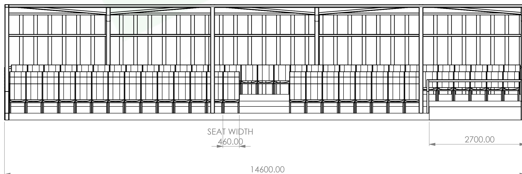
FRONT VIEW
