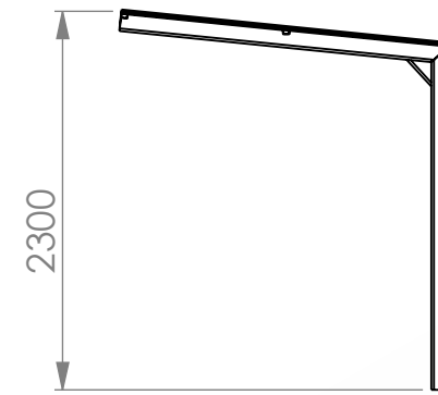
TYPICAL SECTION
