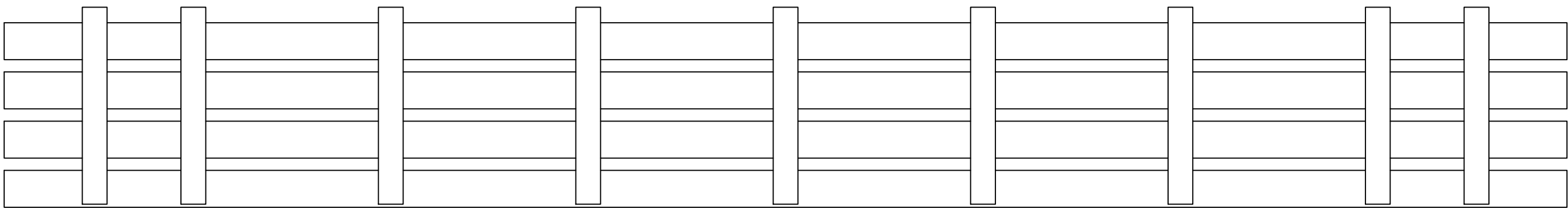
BACKER SYSTEM LAYOUT BACKER DIMENSIONS: 1/2" x 1 1/2" x 12"
