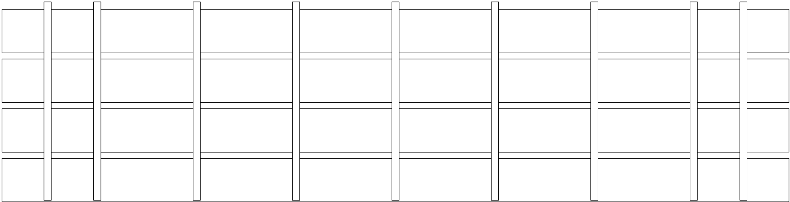
BACKER SYSTEM LAYOUT BACKER DIMENSIONS: 1/2" x 1 1/2" x 12" SCALE REPRESENTATION 1.5 = 12"
