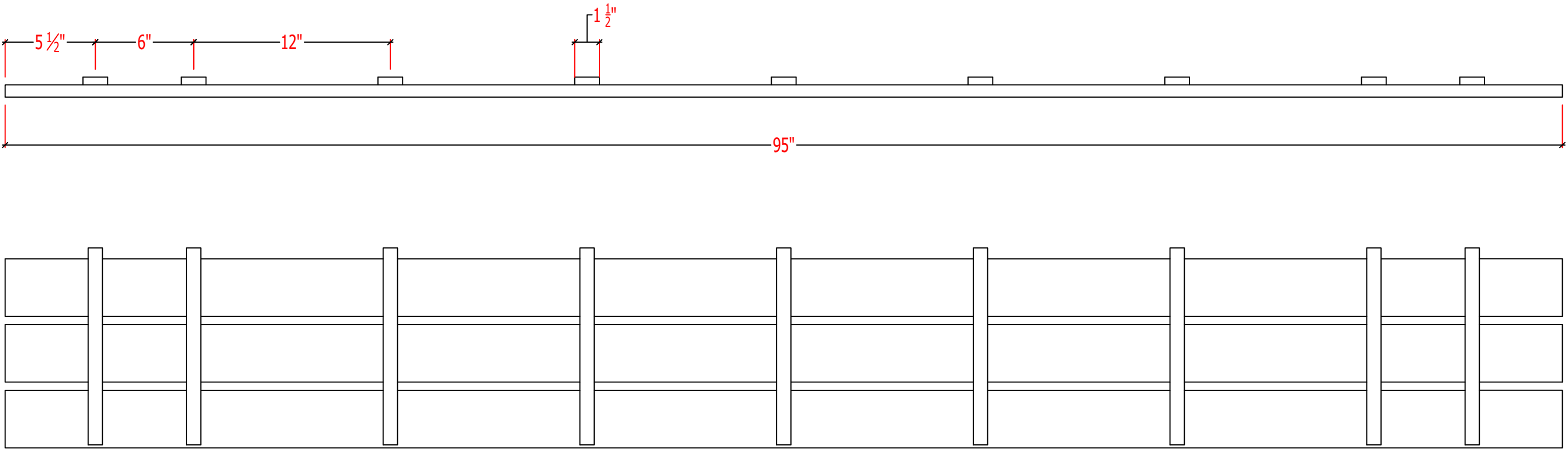
BACKER SYSTEM LAYOUT BACKER DIMENSIONS: 1/2" X 1 1/2" X 12" SCALE REPRESENTATION 1.5 = 12"
