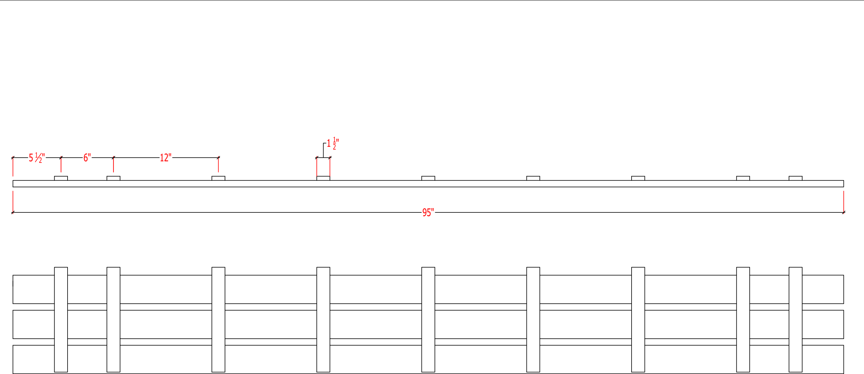
BACKER SYSTEM LAYOUT BACKER DIMENSIONS: 1/2" X 1 1/2" X 12" SCALE REPRESENTATION 1.5 = 12"
