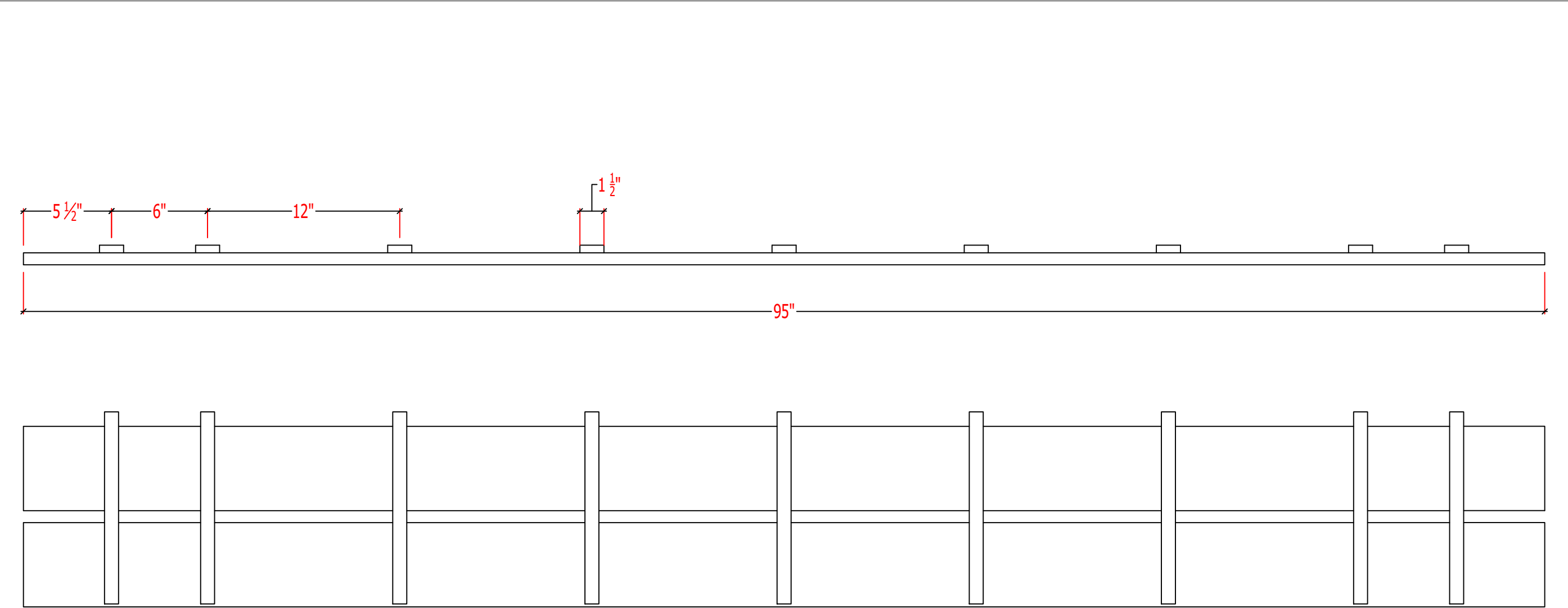
BACKER SYSTEM LAYOUT BACKER DIMENSIONS: \frac{1}{2} " x 1 \frac{1}{2} " x 12"
