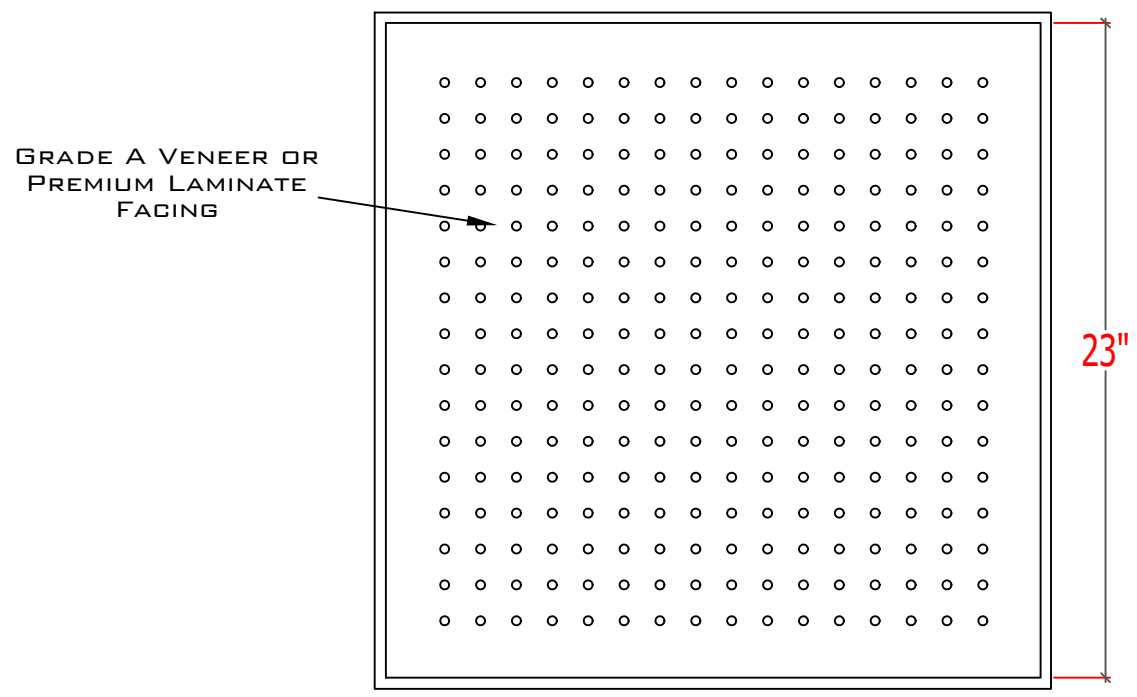
P1 PERFORATION PATTERN 8MM DIAMETER HOLE
