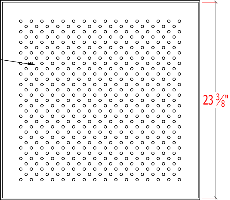
P2 PERFORATION PATTERN 8MM DIAMETER HOLE
