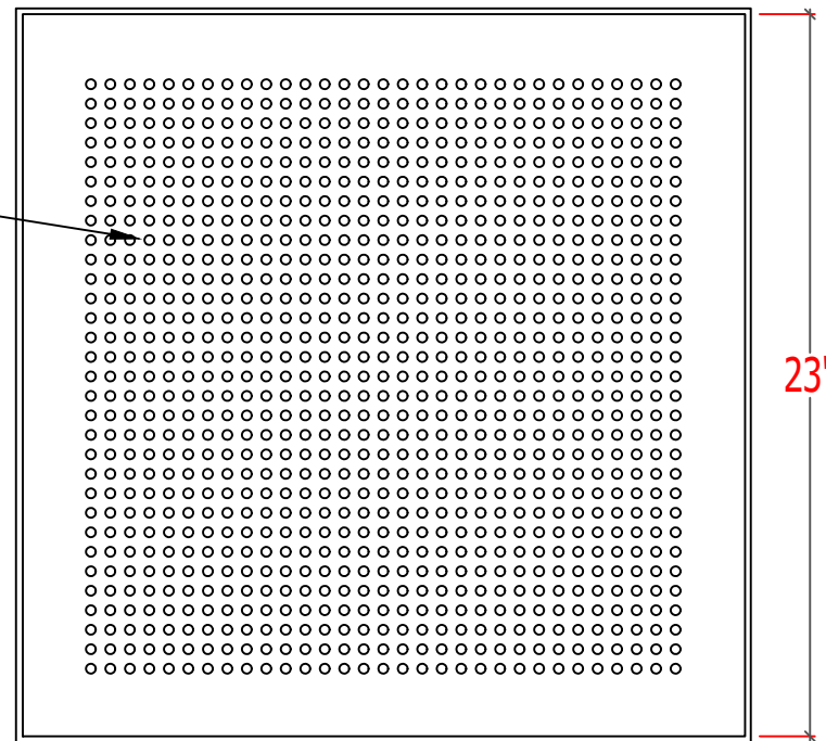
P3 PERFORATION PATTERN 8MM DIAMETER HOLE
