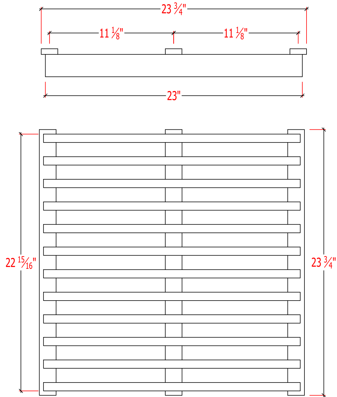
BACKER SYSTEM LAYOUT BACKER DIMENSIONS: 1/2" X 1 1/2" X 23-3/4"
