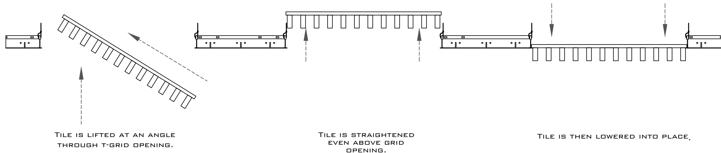
12 BLADE DROP IN PANEL GRILLE PRODUCT REPRESENTATION. ACTUAL BLADE HEIGHT VARIES.
