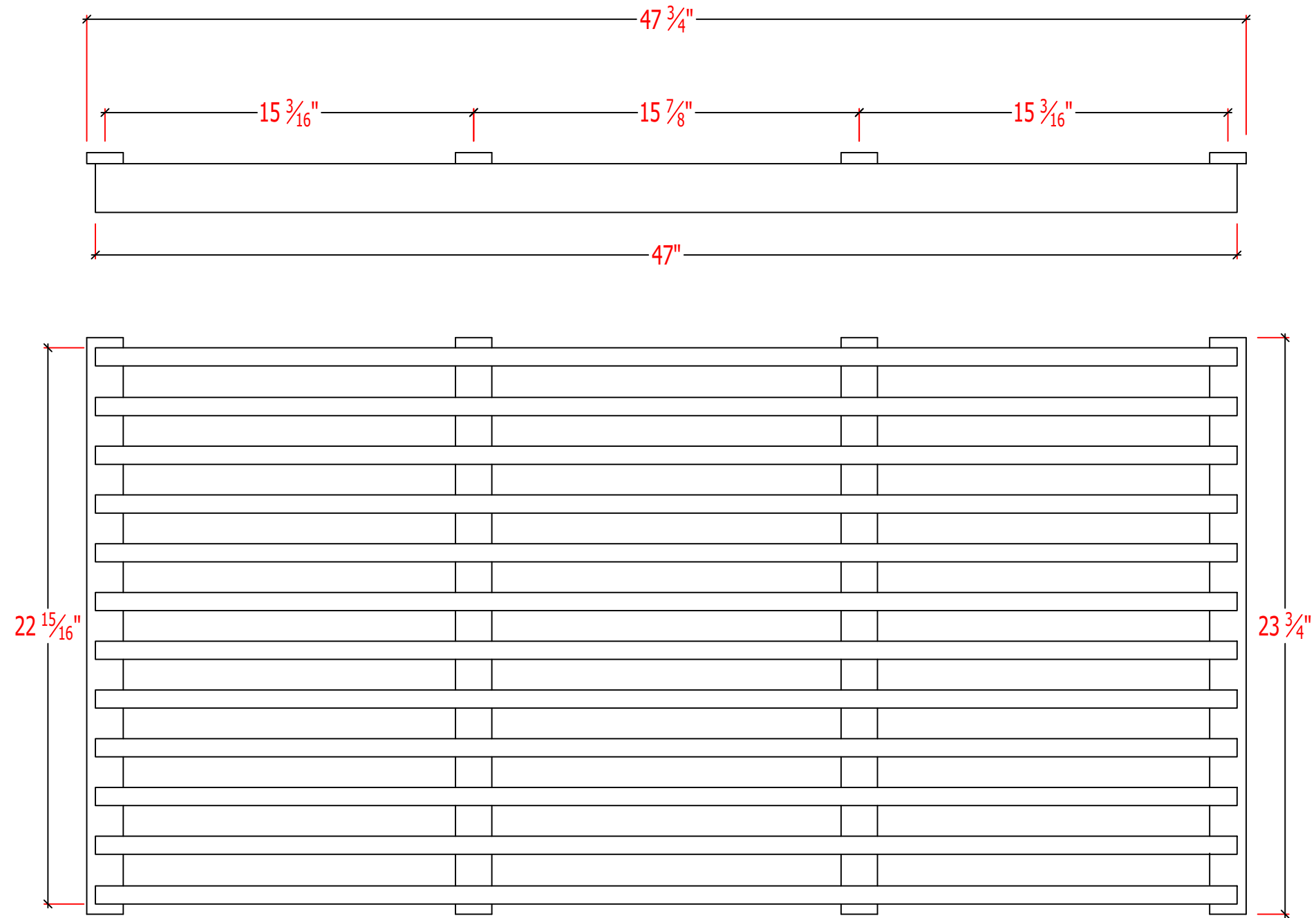
BACKER SYSTEM LAYOUT BACKER DIMENSIONS: 1/2" x 1 1/2" x 23-3/4"
