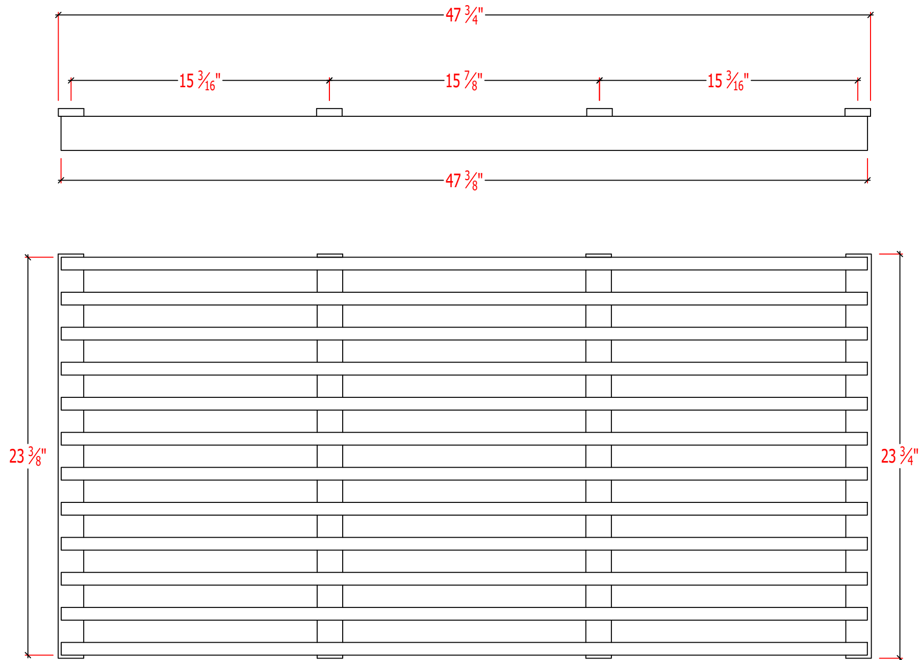
BACKER SYSTEM LAYOUT BACKER DIMENSIONS: 1/2" x 1 1/2" x 23-3/4"
