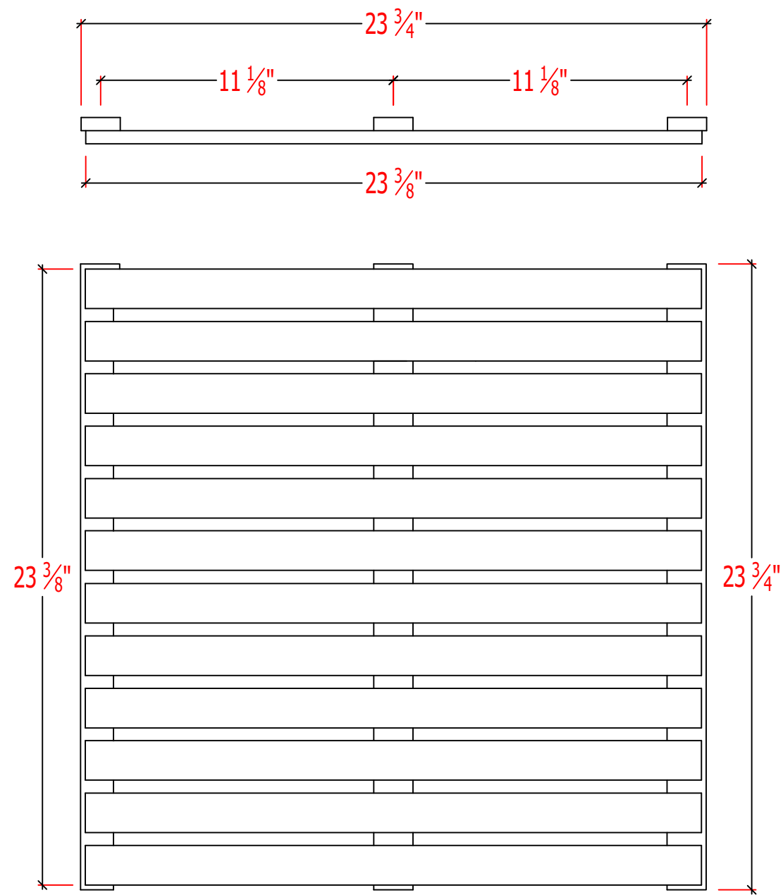
BACKER SYSTEM LAYOUT BACKER DIMENSIONS: \frac{1}{2} " x 1 \frac{1}{2} " x 23 \frac{3}{4} "
