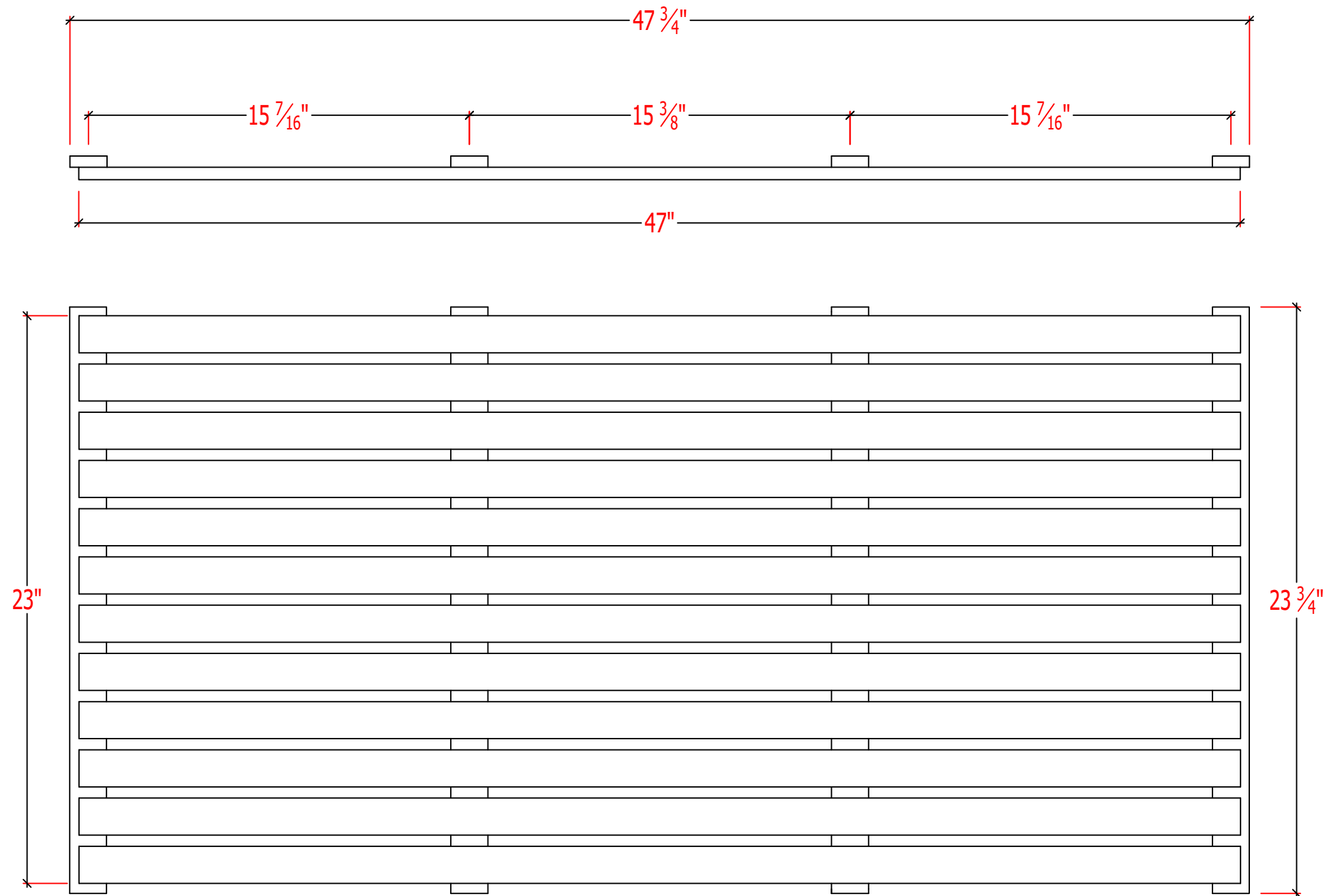
BACKER SYSTEM LAYOUT BACKER DIMENSIONS: \frac{1}{2} " X 1 \frac{1}{2} " X 23 \frac{3}{4} "
