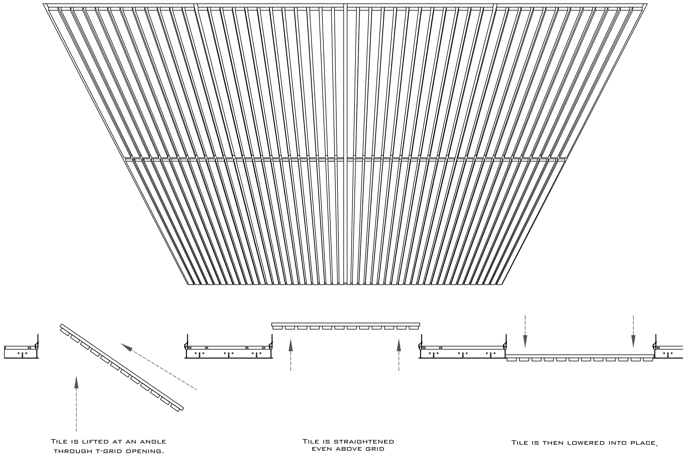
12 BLADE HORIZONTAL DROP IN PANEL GRILLE PRODUCT REPRESENTATION. ACTUAL BLADE WIDTH VARIES.
