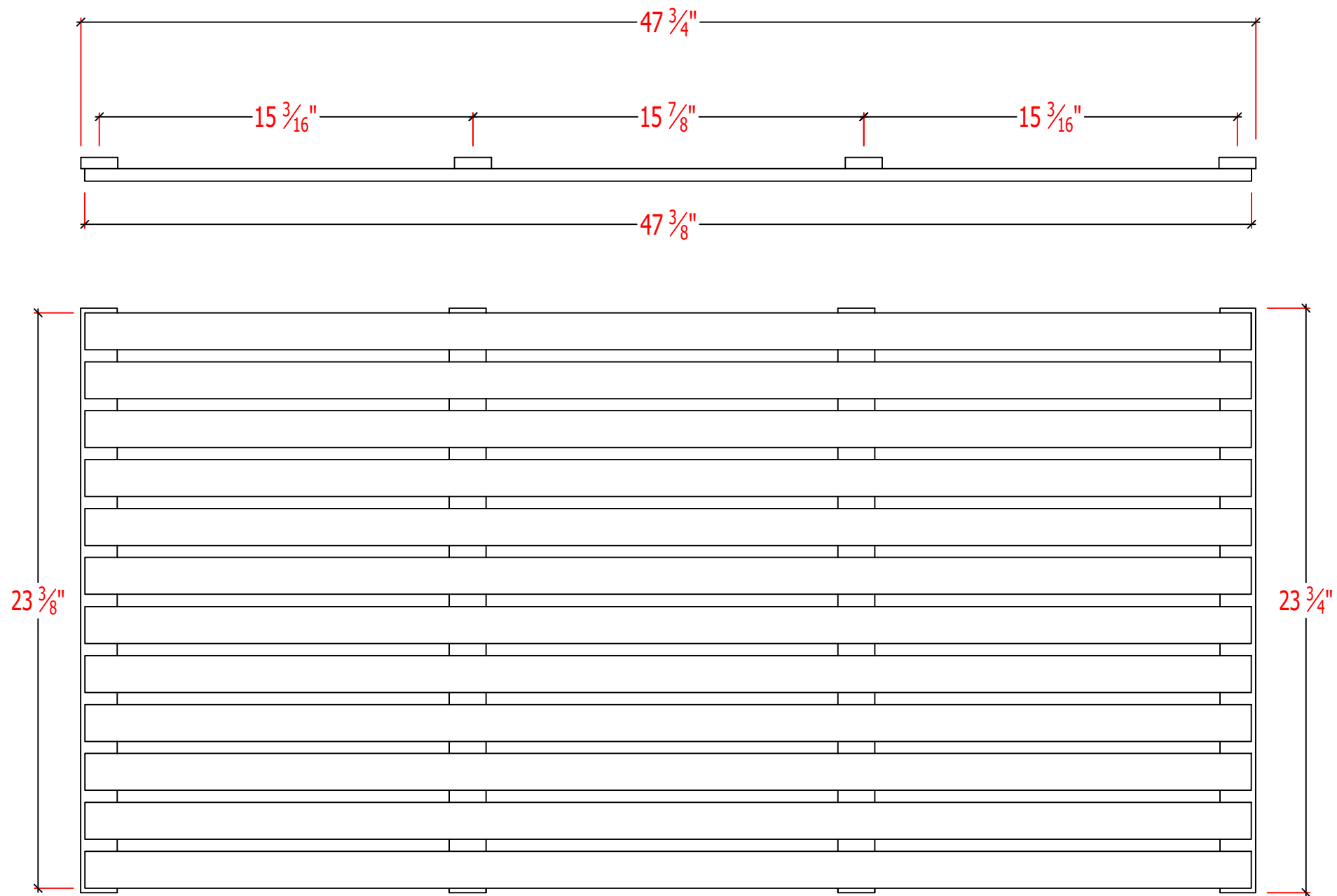
BACKER SYSTEM LAYOUT BACKER DIMENSIONS: 1/2" x 1 1/2" x 23-3/4"
