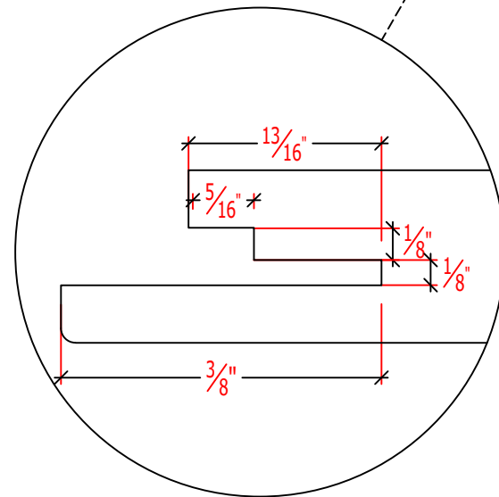
PROFILE C
