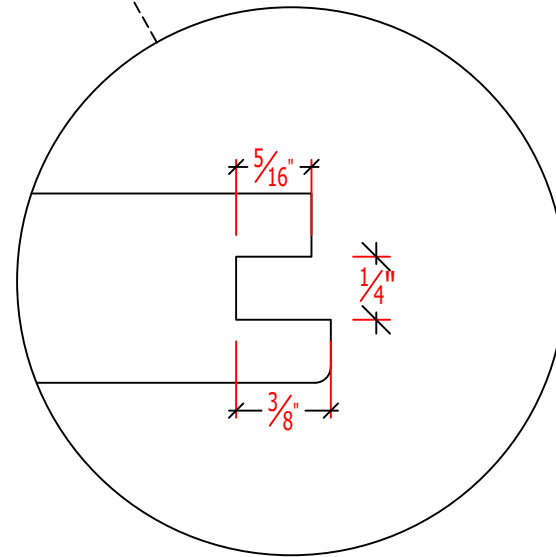
PROFILE D
