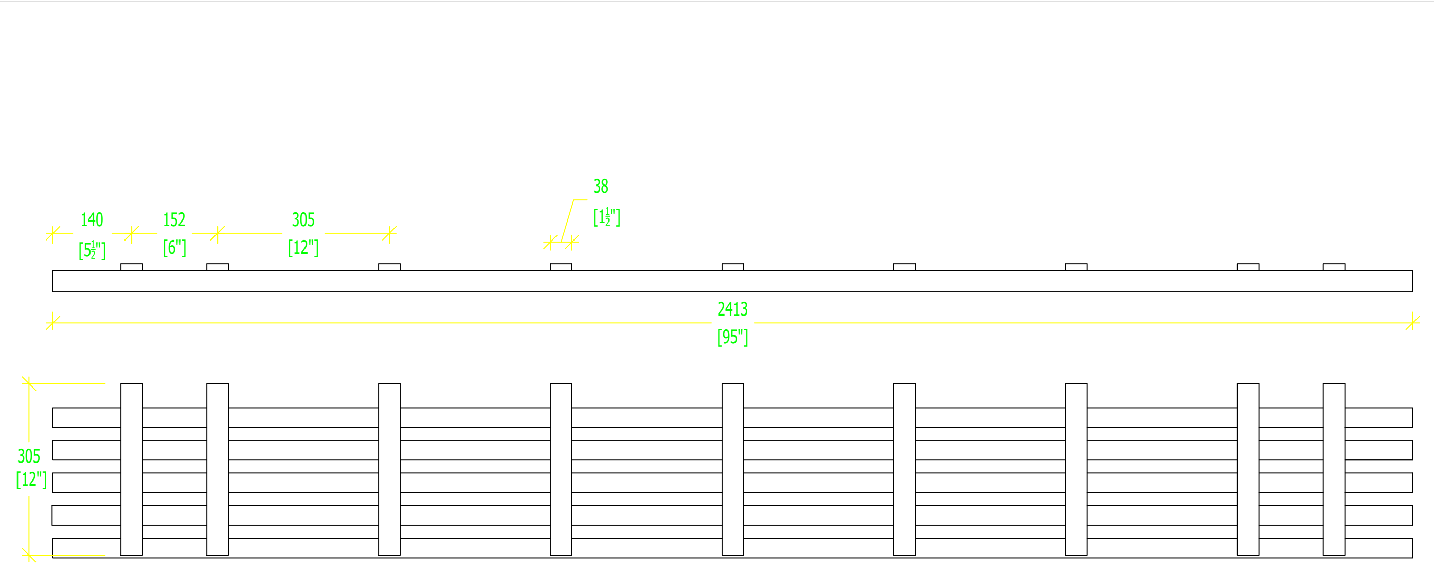
BACKER SYSTEM LAYOUT BACKER DIMENSIONS: ½" x 1 ½" x 12" Scale representation 1.5 = 12"
