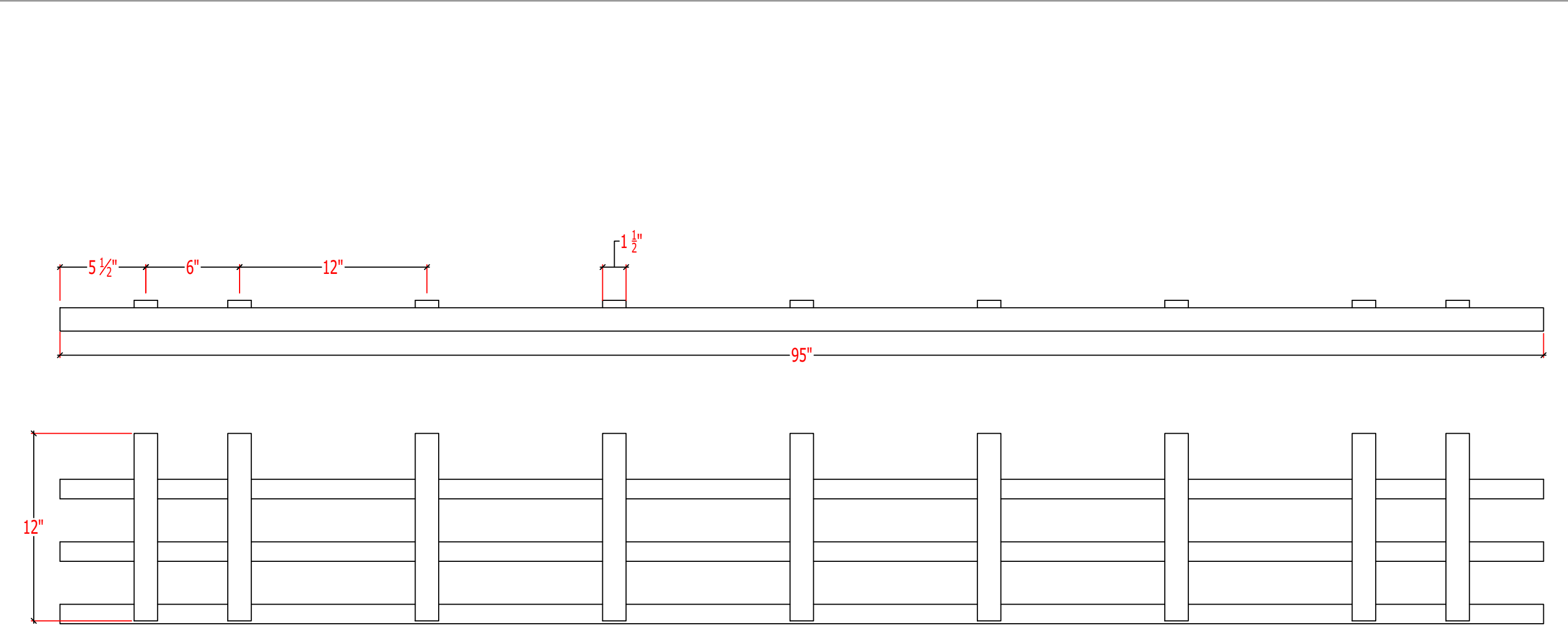
BACKER SYSTEM LAYOUT BACKER DIMENSIONS: 1/2" x 1 1/2" x 12"
