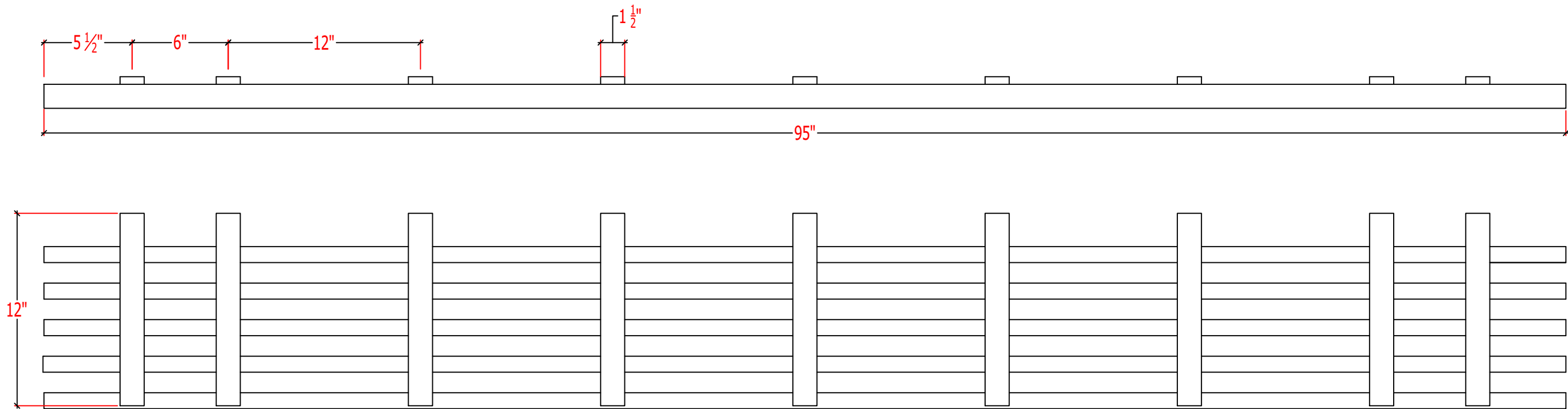
BACKER SYSTEM LAYOUT BACKER DIMENSIONS: 1/2" x 1 1/2" x 12"
