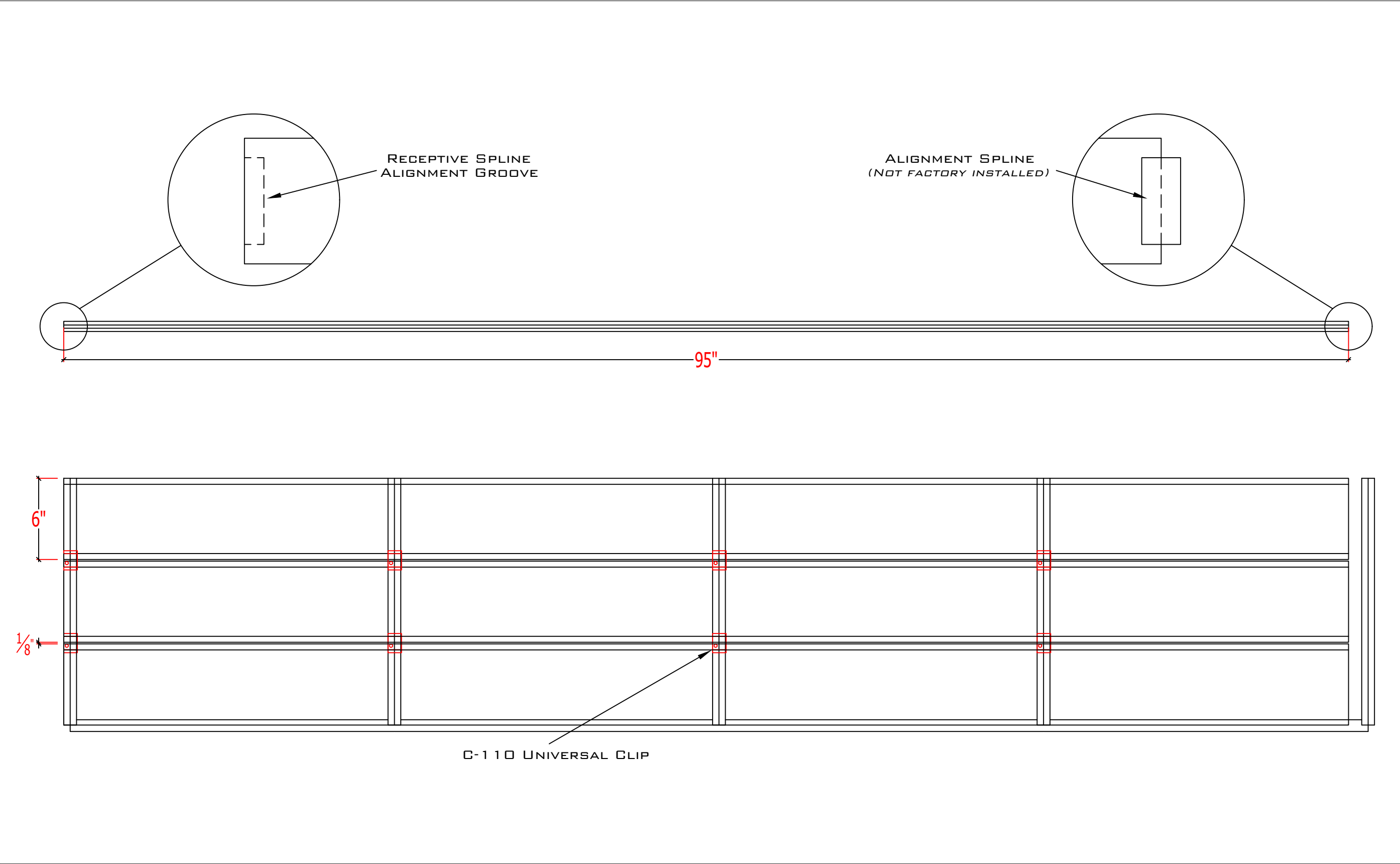
1.2 Clip Configuration
