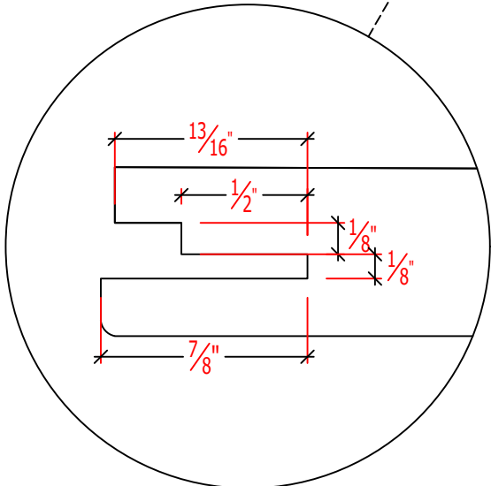
PROFILE A
