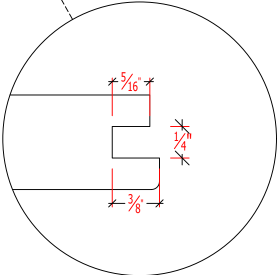
PROFILE D
