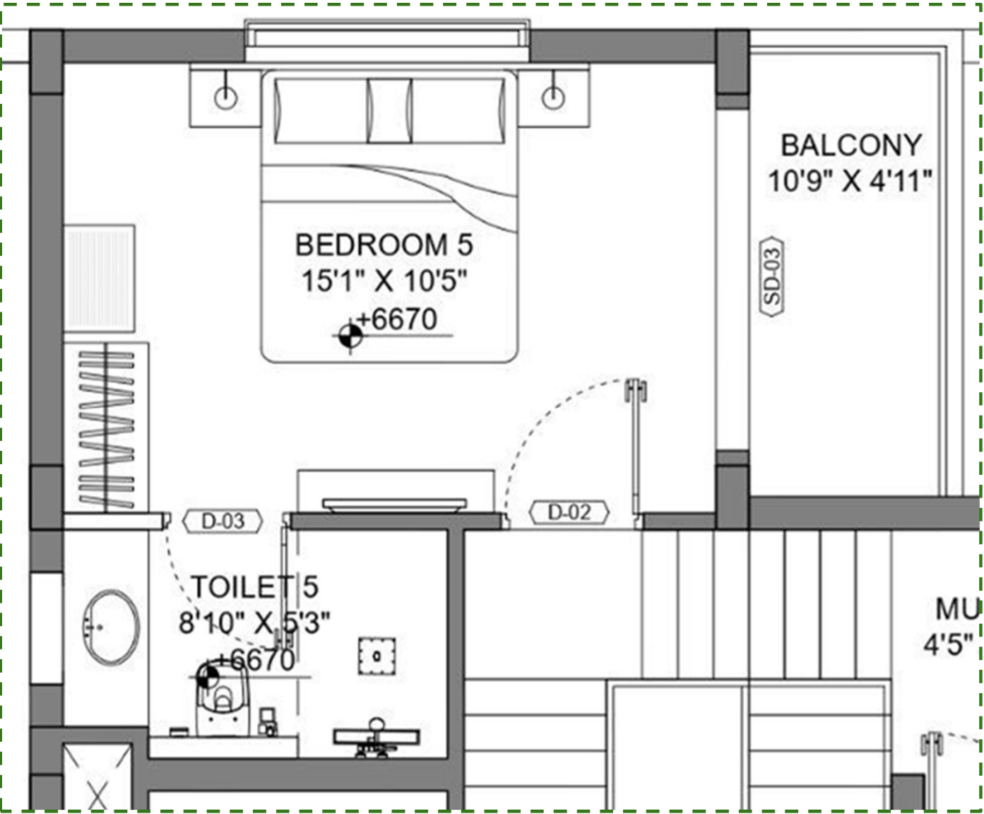
BEDROOM 5 - TERRACE
