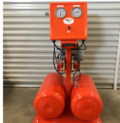
RTM# 6200-01 Composites One# 693670 VacPack Dual Vac Rotary Vane Electric with Tanks & Cart
