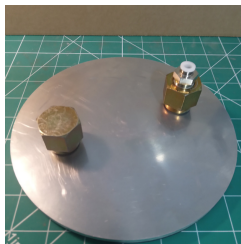
RTM# 4578-01 Composites One# 695121 Lid for Vacuum Bowl Aluminum with Assembly 1/4"
