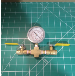
RTM# 4760-02 Composites One# xxxxxx Ball Valve Assembly with Vacuum Gauge Liquid Filled 2" Replacement
