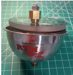
RTM# 4560-01 Composites One# 527357 Vacuum Bowl with Insert, Lid Lexan with Assembly 1/4"
