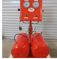
RTM# 6500-01 Composites One# 701072 VacPack 24 V High Flow Venturi Dual Vac with Tanks & Cart
