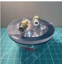
RTM# 4575-05 Composites One# 591047 Vacuum Bowl & Lid Lexan with Assemblies 1/2"
