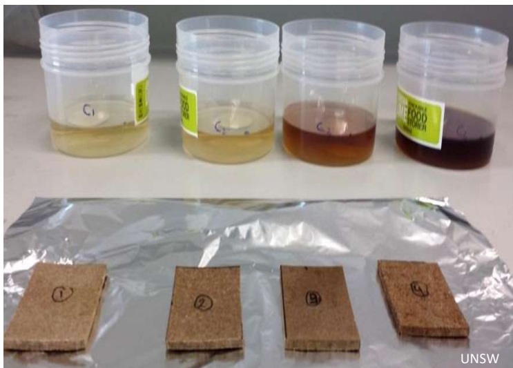
Demonstration by University of New South Wales (UNSW) researchers showing various particleboards made from brown seaweed and mollusc waste.
