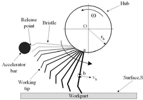
Figure 15 - Acceleration of the bristle tip towards the target surface upon release from the accelerator bar.
