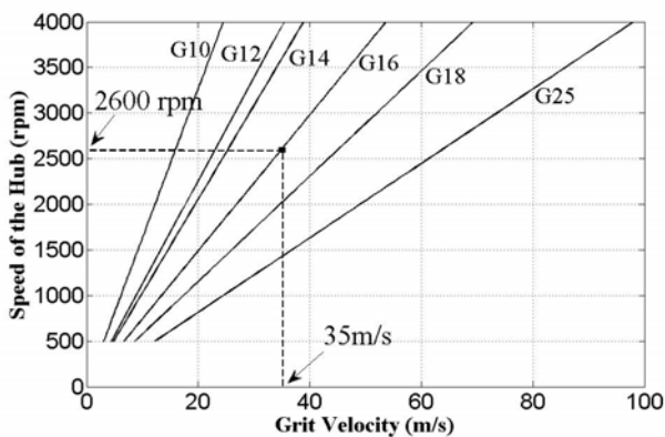
Figure 13 - Relationship between spindle speed and grit velocity for several different steel media for the case of standard bristle motion. (Note: spindle speed 2600 rpm corresponds to grit velocity of 35 m/s for G16)
