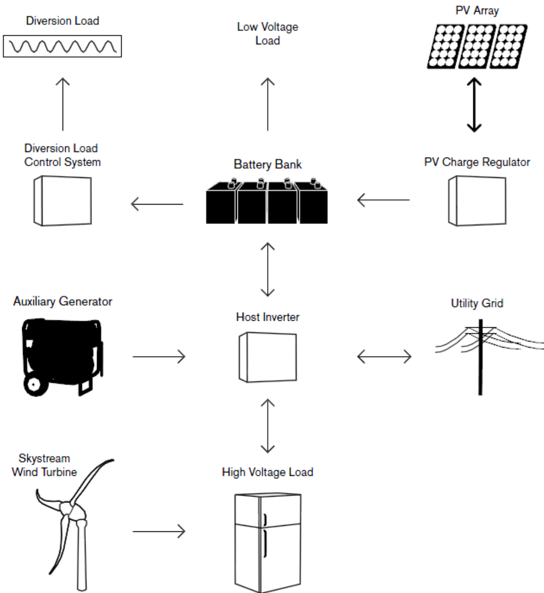
Figure 1: Typical elements of a battery charging system
