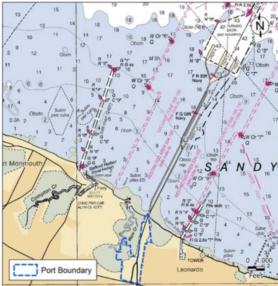
Figure 42: Naval Weapons Station Earle - NOAA Depth Chart
