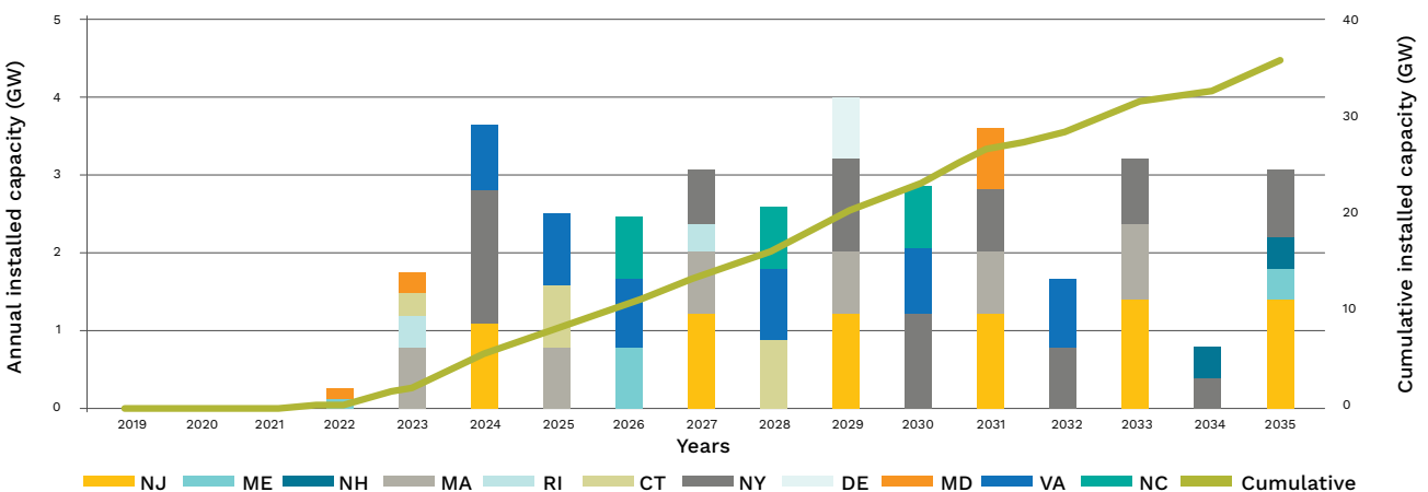
FIGURE 1-1: SHARE OF EAST COAST MARKET
