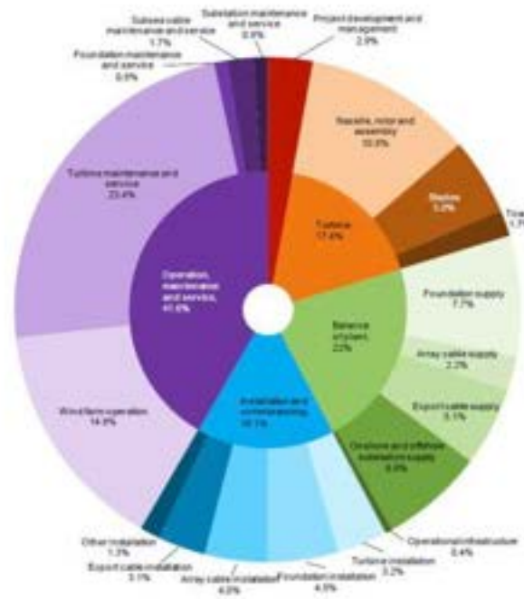
CAPEX and OPEX breakdown of an offshore wind farm
