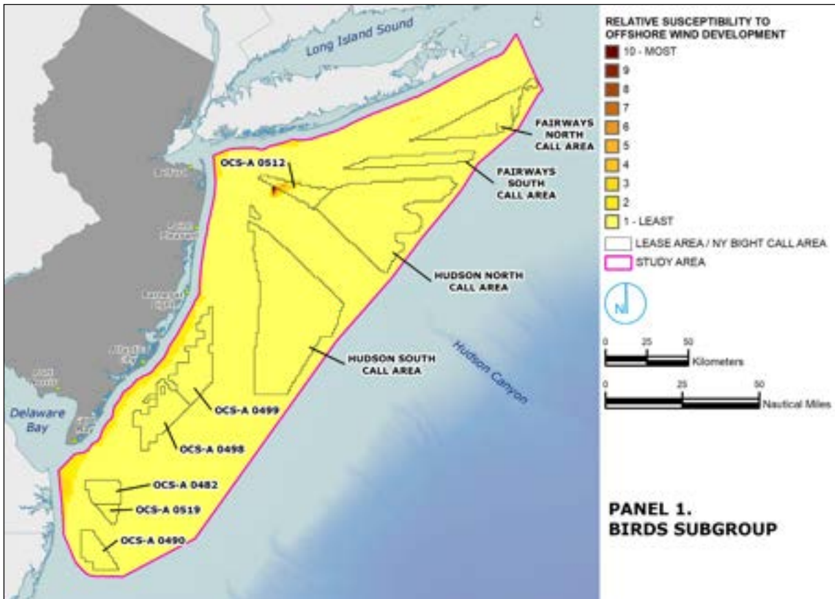
FIGURE 2-1: RELATIVE SUSCEPTIBILITY OF BIOLOGICAL RESOURCE SUBGROUPS TO OFFSHORE WIND DEVELOPMENT
