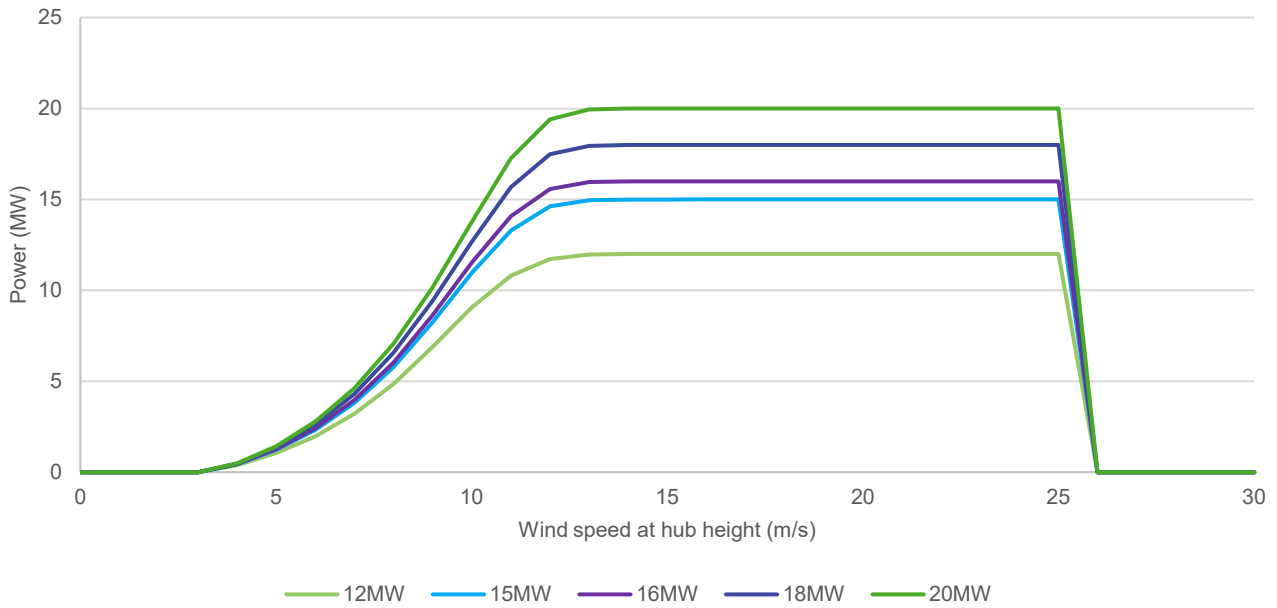
Figure 2: Power curves used to derive energy production.
