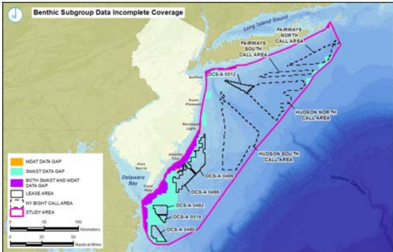
Figure 7: Benthic Subgroup Data Incomplete Coverage
