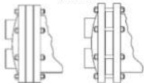
Full Face Boltless Tube Sheet
