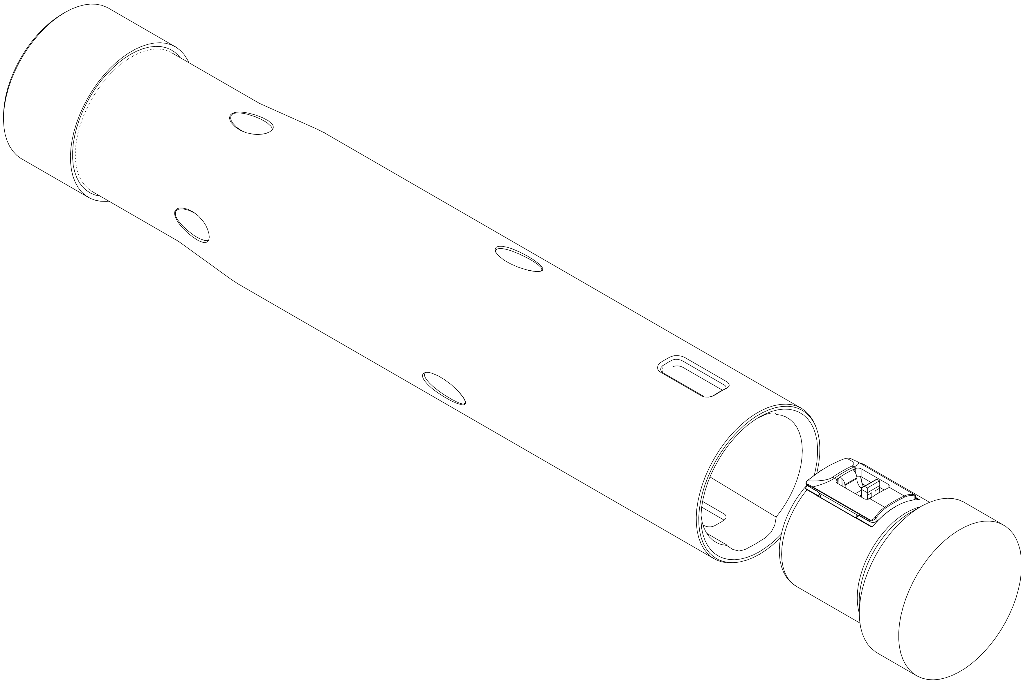
2. ALIGN RETENTION SNAPS TO GUIDE GROOVES
