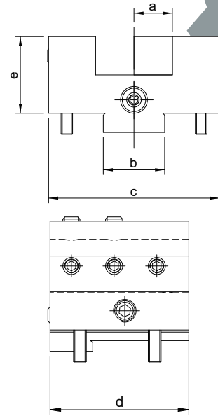
Facing tool holder
