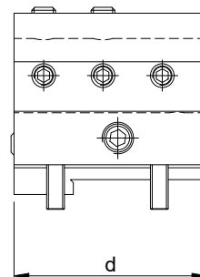
Facing tool holder
