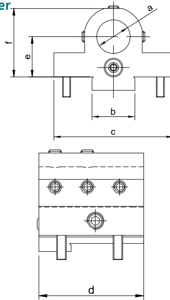
Boring bar tool holder
