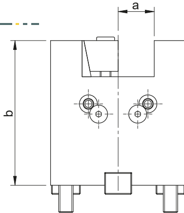
Facing Tool holder
