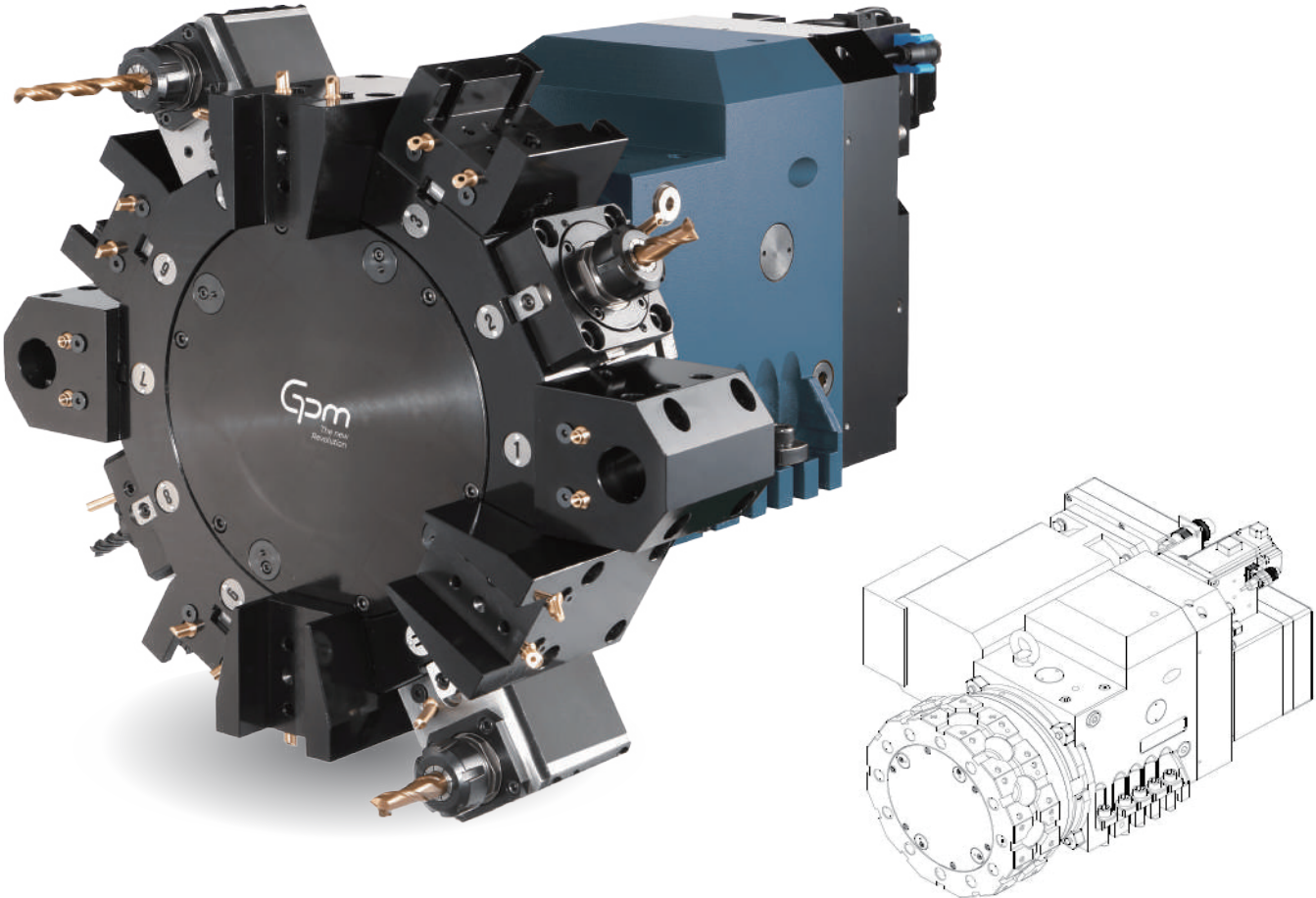
動力刀馬達 - U型連結 Tool drive motor – U-shape connection
