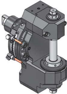
Gear Hobbing unit
