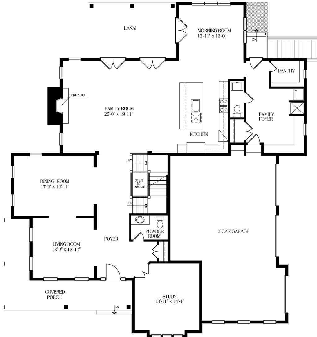
LOWER FLOOR PLAN 2345 SF
