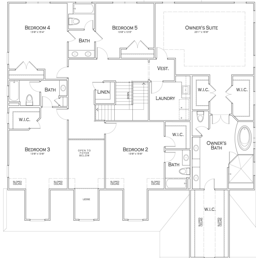
SECOND FLOOR PLAN 2,560 Sq.Ft.
