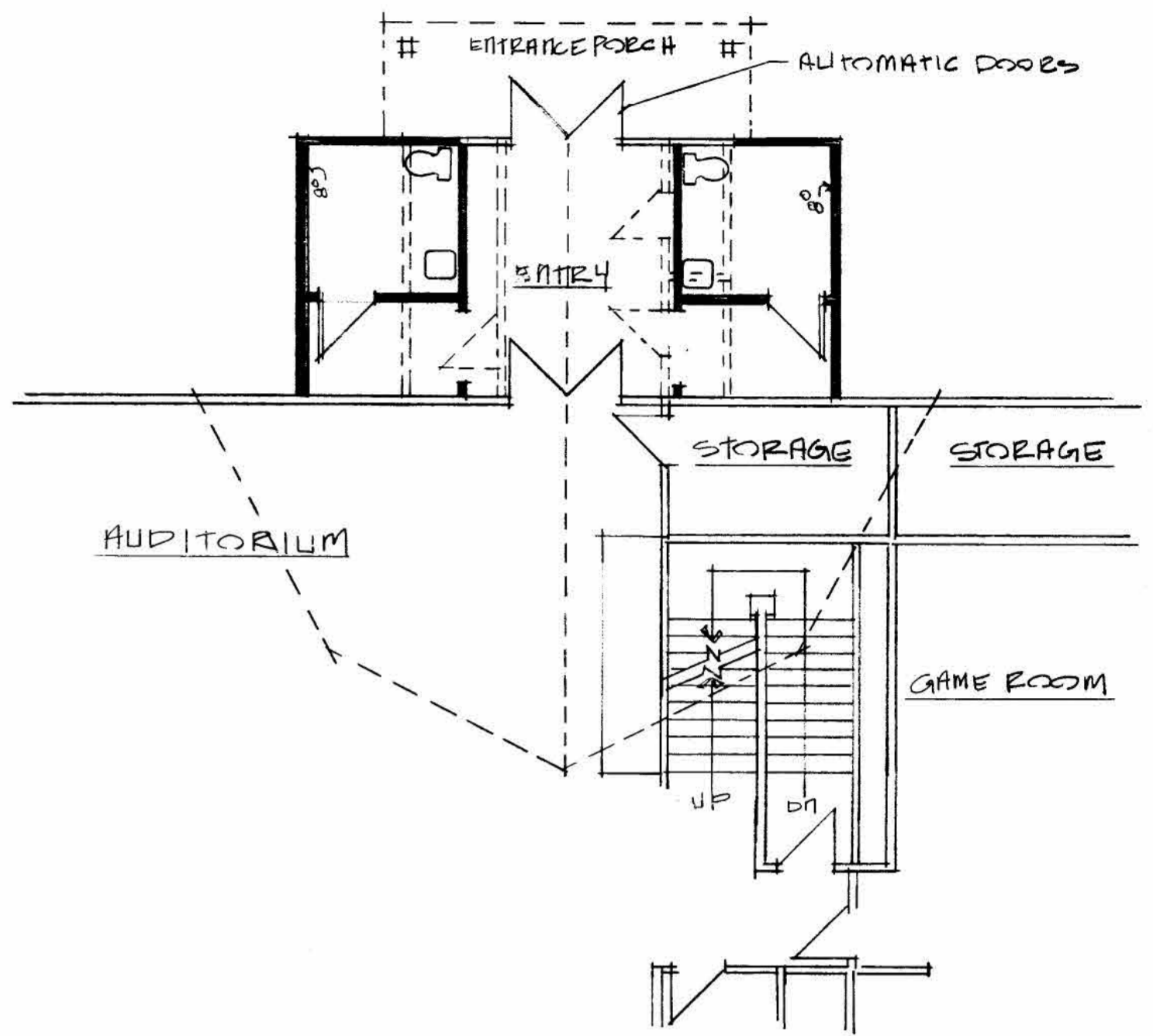
OPTIONAL ENTRANCE LAYOUT 1/8"=1'-0"
