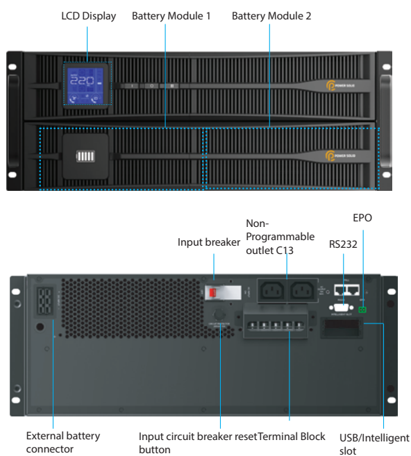
6KVA Rear Panel
