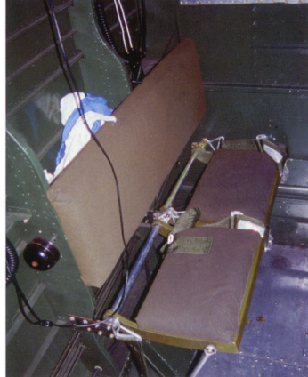
(Right) The waist gunners ride-along seat is located on the port side of the fuselage, just aft of the bomb bay. The round, black object at the left is a throwback to a bygone era...an ashrtry! (Lou Drendel)
