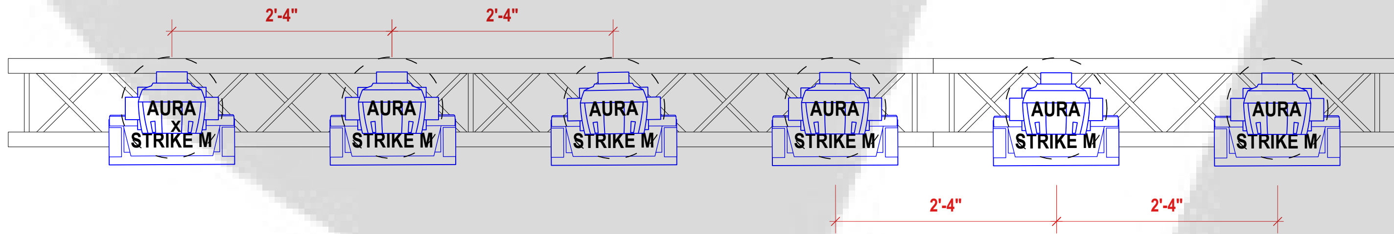
USR, USL, DSR, DSL TRUSS POSITION FIXTURE DETAIL SCALE: 1"=1'0"
