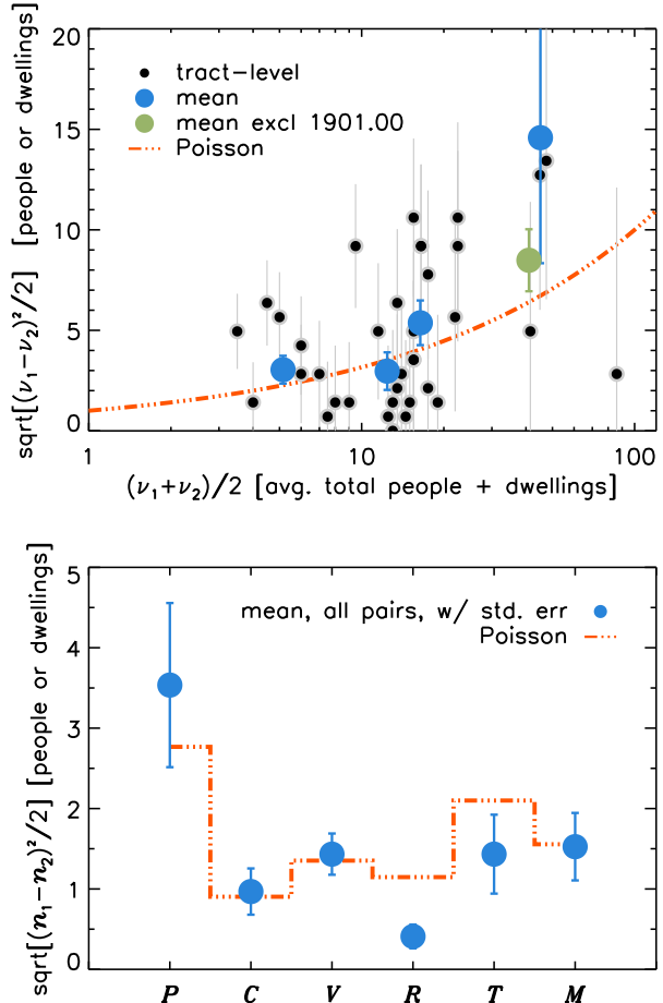
Figure 2: Intercouter result comparisons. Top: mean tract-level differences (large blue points; 10-pair bins) are 1.4\times the Poisson expectation (dot-dashes; \sqrt{\langle v \rangle} ); 1.3\times excluding outlier tract 1901.00 (large green point). Small points show pairwise differences. Bottom: mean category-level dispersions are consistent with random errors except for RVs, which are identified significantly more consistently. Only means are shown at bottom to reduce clutter.
