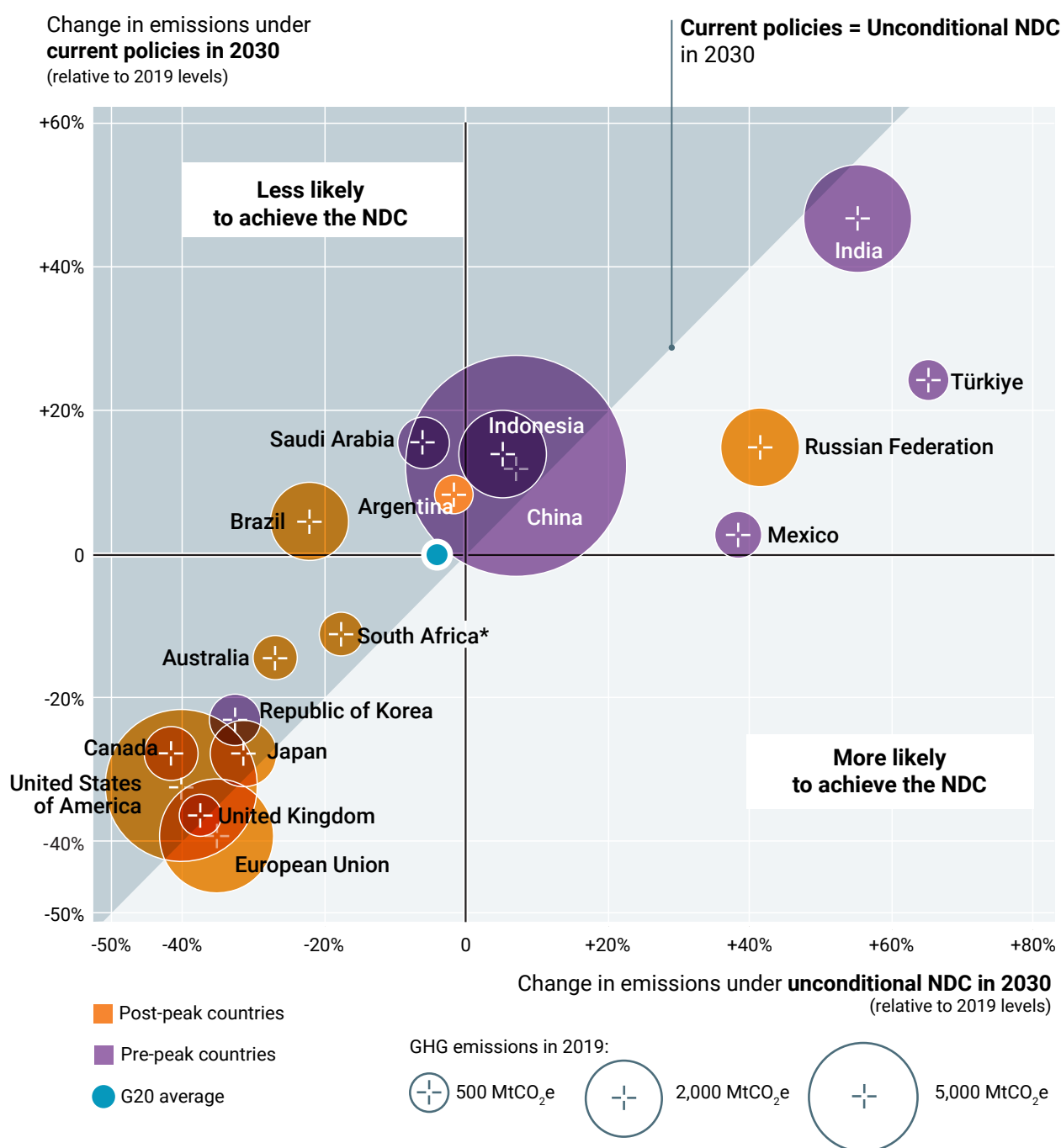
Figure 3.2 The landscape of current NDC targets and implementation gaps for the G20 members collectively and individually by 2030, relative to 2019 emissions
