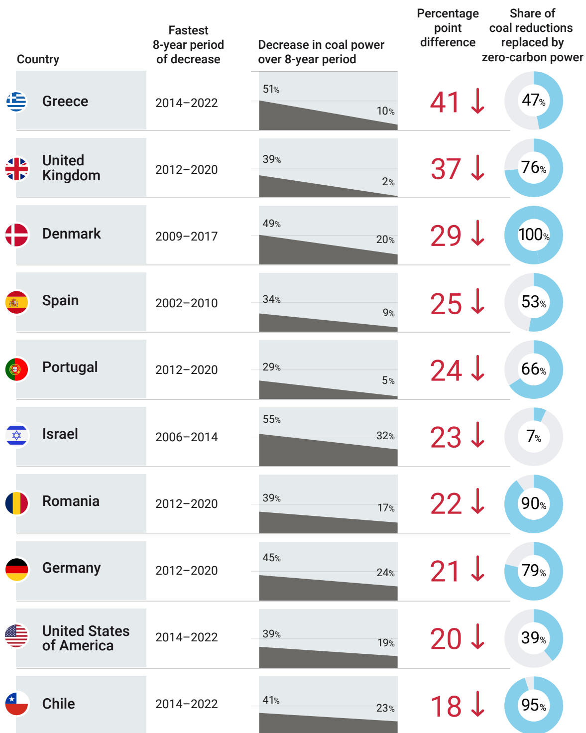
Figure B6.2 Fastest eight-year periods of reductions in the share of coal in electricity generation
