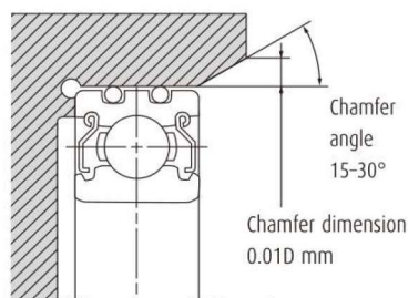
Fig. 5 Housing shape and dimension
