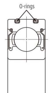
Fig. 1 Structure of Creep-Free Bearings
