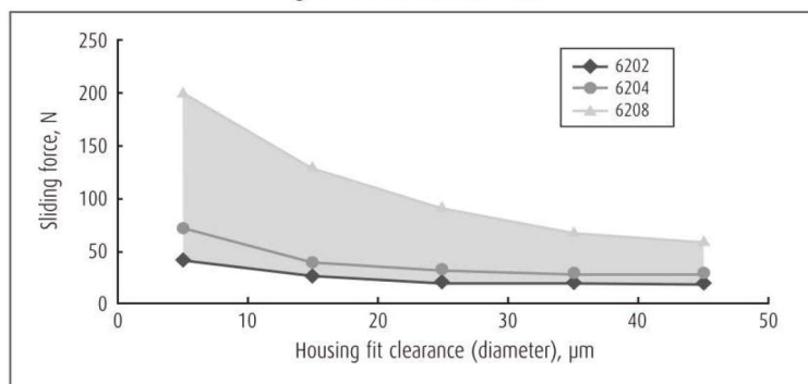
Fig. 4 Fit and sliding force
