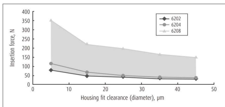
Fig. 3 Fit and insertion force
