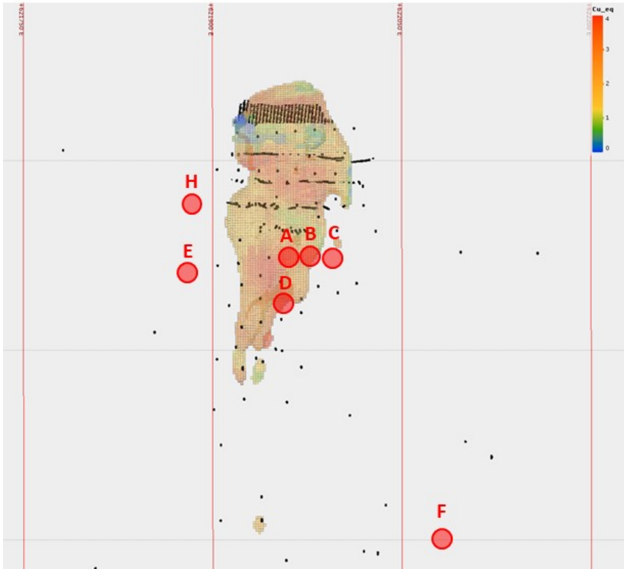
Figure 7.14 Longitudinal section sketch of the Fabie Bay deposit looking north showing the Cu equivalent grade and proposed Phase One (Holes A through E) and Phase Two drill holes (F & H). Compiled by Electro Metals, March, 2022. The sketch illustrated the relative intensity of mineralization. Metal prices and estimates of recoveries as follows: Copper $3.26/lb 80%, zinc $1.24 per pound 72%, gold $1626 per oz 60%, silver $20.71 per oz 40% - prices are three – year look back prices as at March 2022, recoveries are conservative estimates as agreed with management for potential payable recoveries. Cu-eq calculation: [(\text{Cu Grade} \times \text{Cu Price} \times \text{Cu Rec}) + (\text{Zn grade} \times \text{Zn Price} \times \text{Zn Rec}) + (\text{Ag Grade} \times \text{Ag Price} \times \text{Ag Rec}) + (\text{Au grade} \times \text{Au Price} \times \text{Au Rec})] / \text{Cu Price} / 22.046 , where Rec = potential recovery estimated to the best of management's and Author's knowledge.
