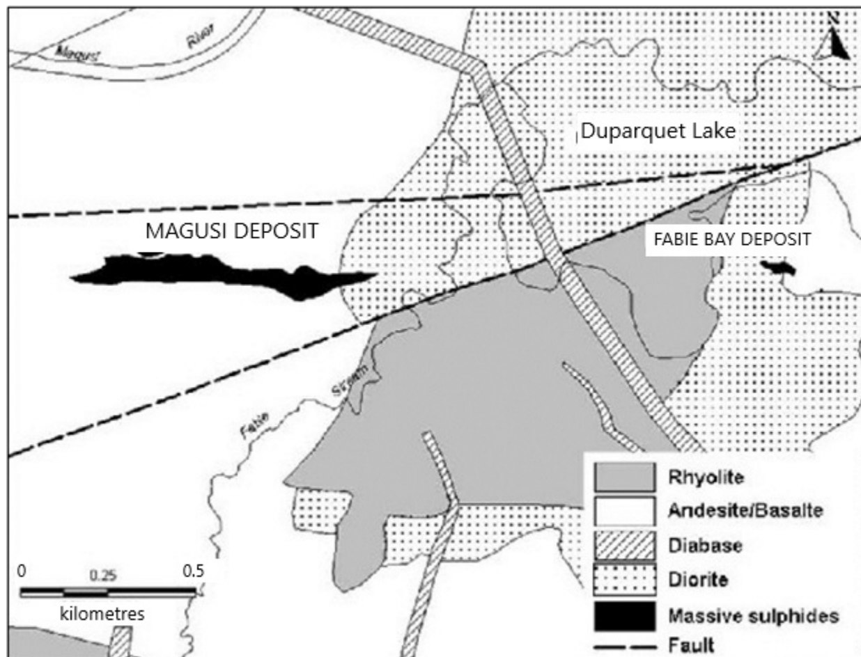
Figure 7.6 Local geology of the project area sketch extracted from 2005 Cheng et. al. Note the rhyolite and diorite masses between Fabie and Magus deposits. There has been limited exploration in this gap area.
