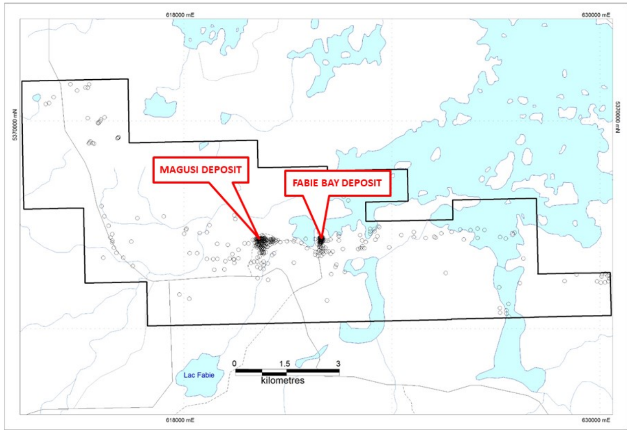
Figure 6.3 Map showing location of historic drill hole collars within the Property. Compiled by Electro Metals, March 2022. North is to the top of the diagram.
