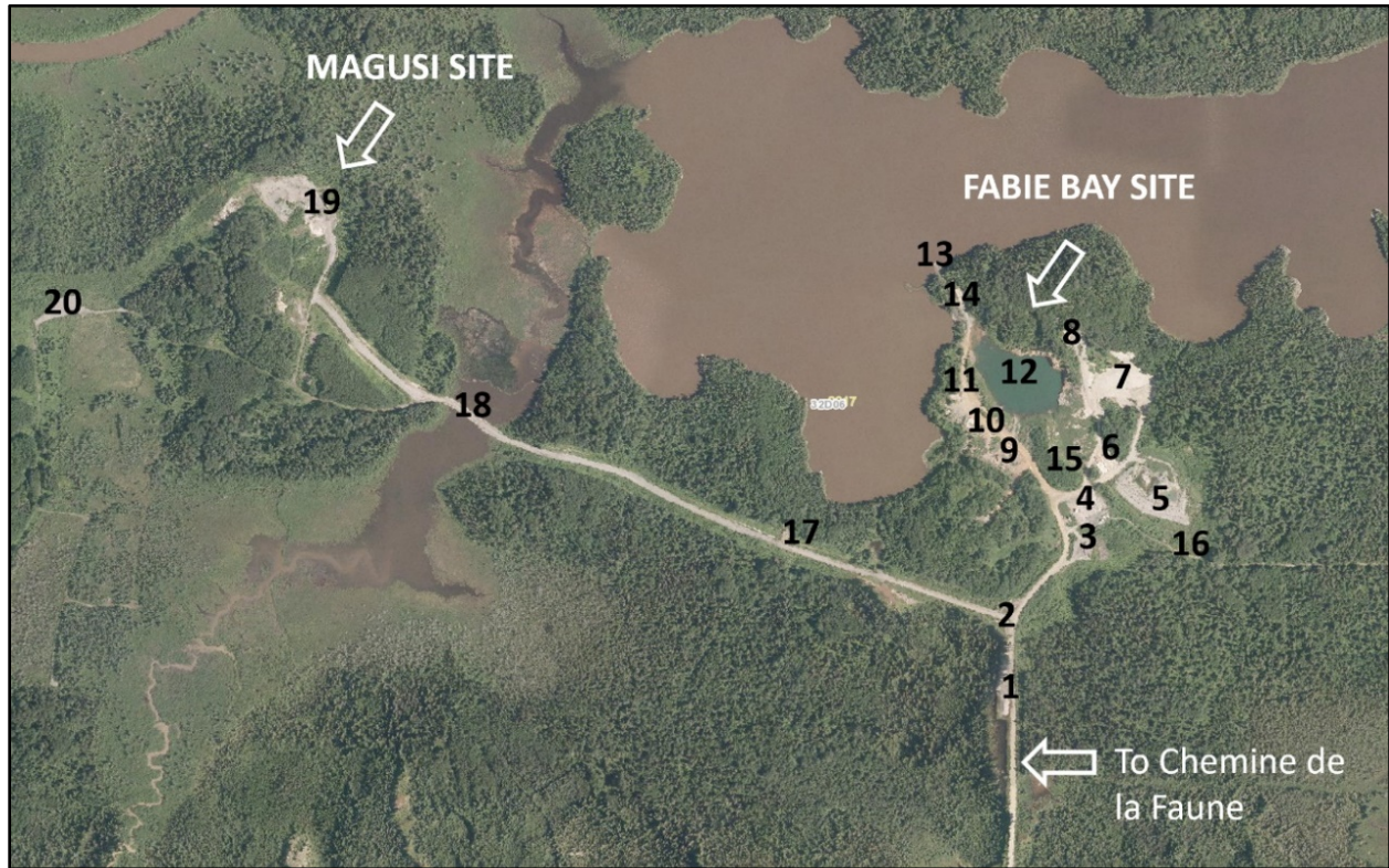
Figure 4.3 Google Earth image of the historic Magusi and Fabie Bay deposit areas showing remaining infrastructure. Compiled March, 2022, Google Earth, North is to the top of the image. Distance across the image is 2.5 km.
