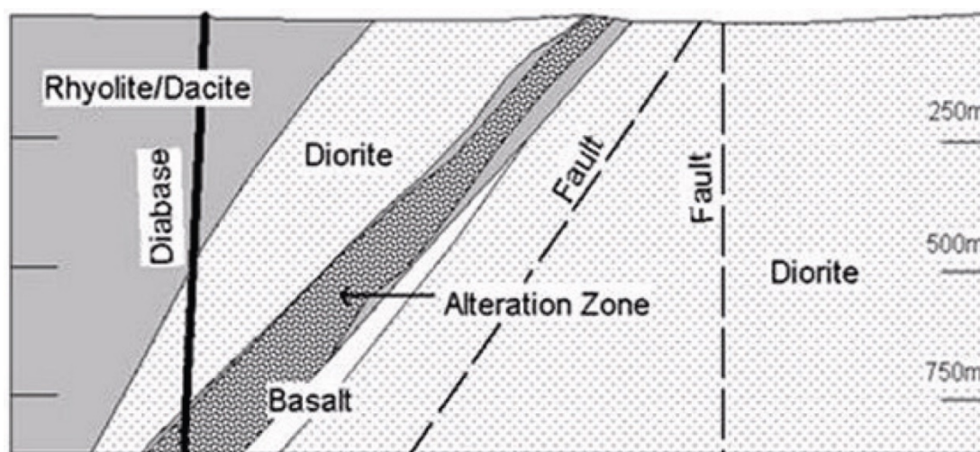
Figure 7.10 Typical cross section through the Fabie Bay deposit looking west. (2005, Cheng et. Al.)
