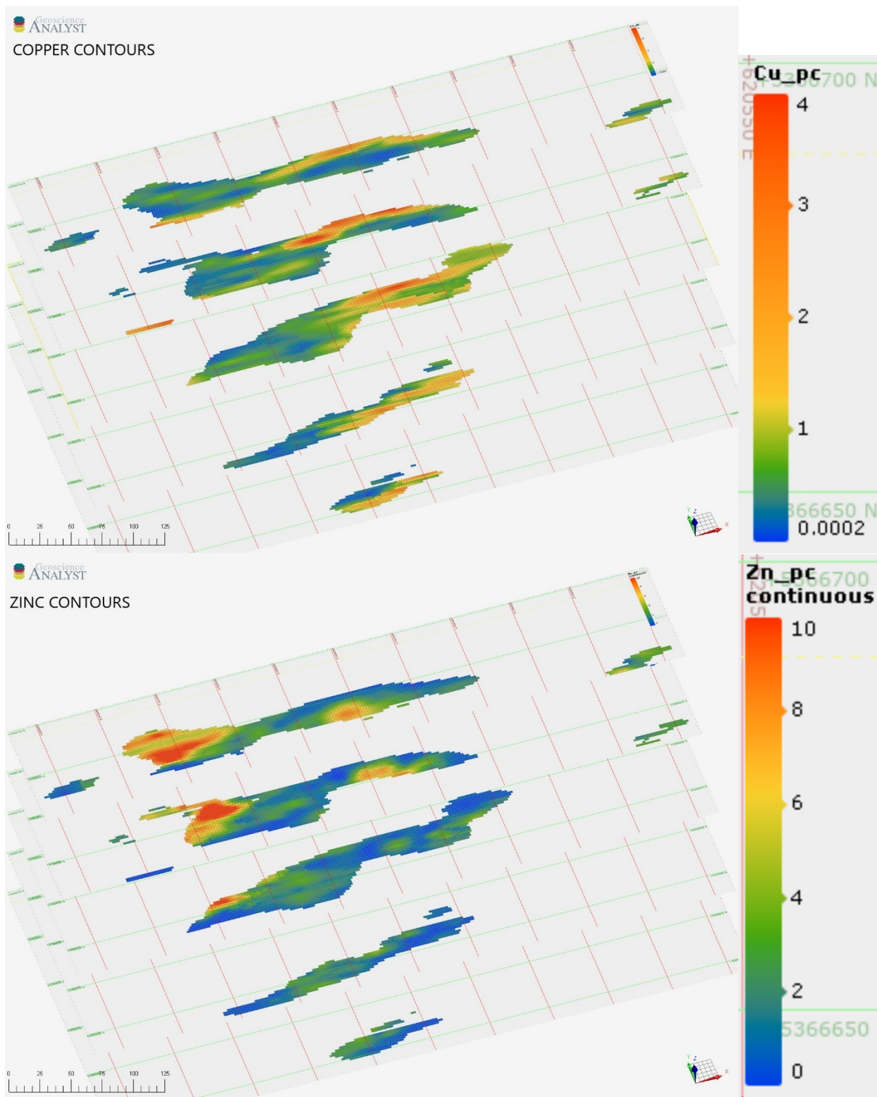
Figure 7.9 Thematic diagram of contoured plan slices of the Magusi massive sulphide showing the separate relative Cu-rich and Zn-rich areas of the deposit at increasing depths, levels 225, 175, 125, 75 and 25 metre depths. Looking North. Compiled by Electro Metals, March 2022.
