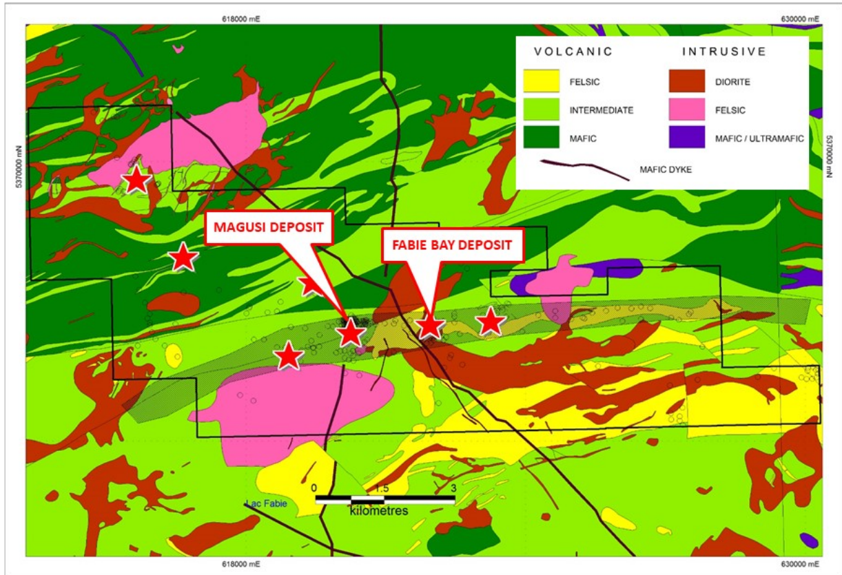
Figure 7.5 Regional geology of the project area, Property outline, and location of the Magusi and Fabie Bay deposits showing initial target locations and trend of the “favourable horizon”, as of December 2022. (2022, Québec Government SIGEOM website)
