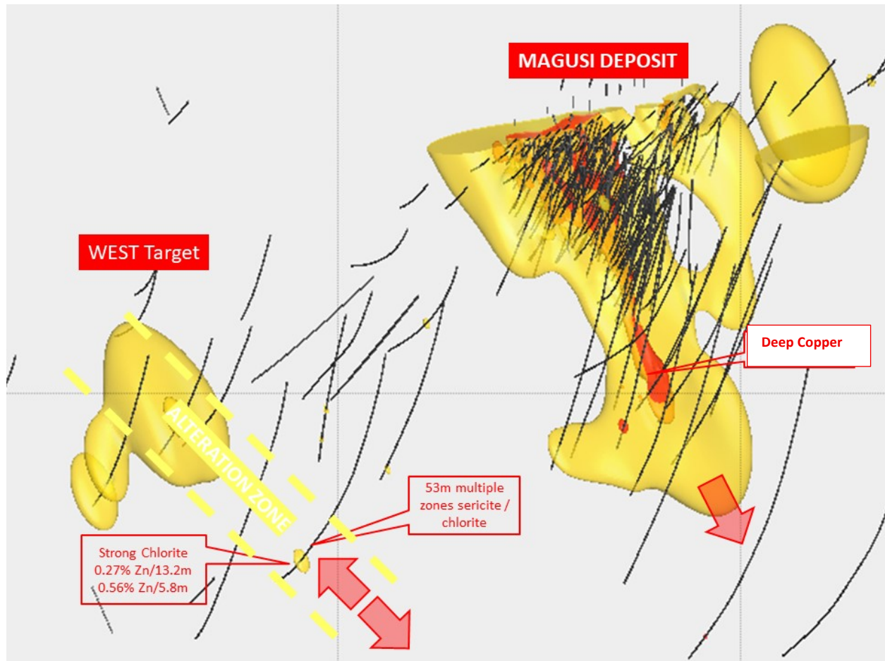
Figure 7.15 ISOMETRIC DIAGRAM looking northeast illustrating the relative position of the Magusi deposit and interpreted West target VMS alteration zones (based on historic compilation), outlined as golden objects. The West target is recommended for further drill testing; located immediately west of the Magusi VMS deposit and its associated alteration zone. Compiled by Electro Metals, March, 2022. Vertical grid lines are 1,000 metres apart on the horizontal.
