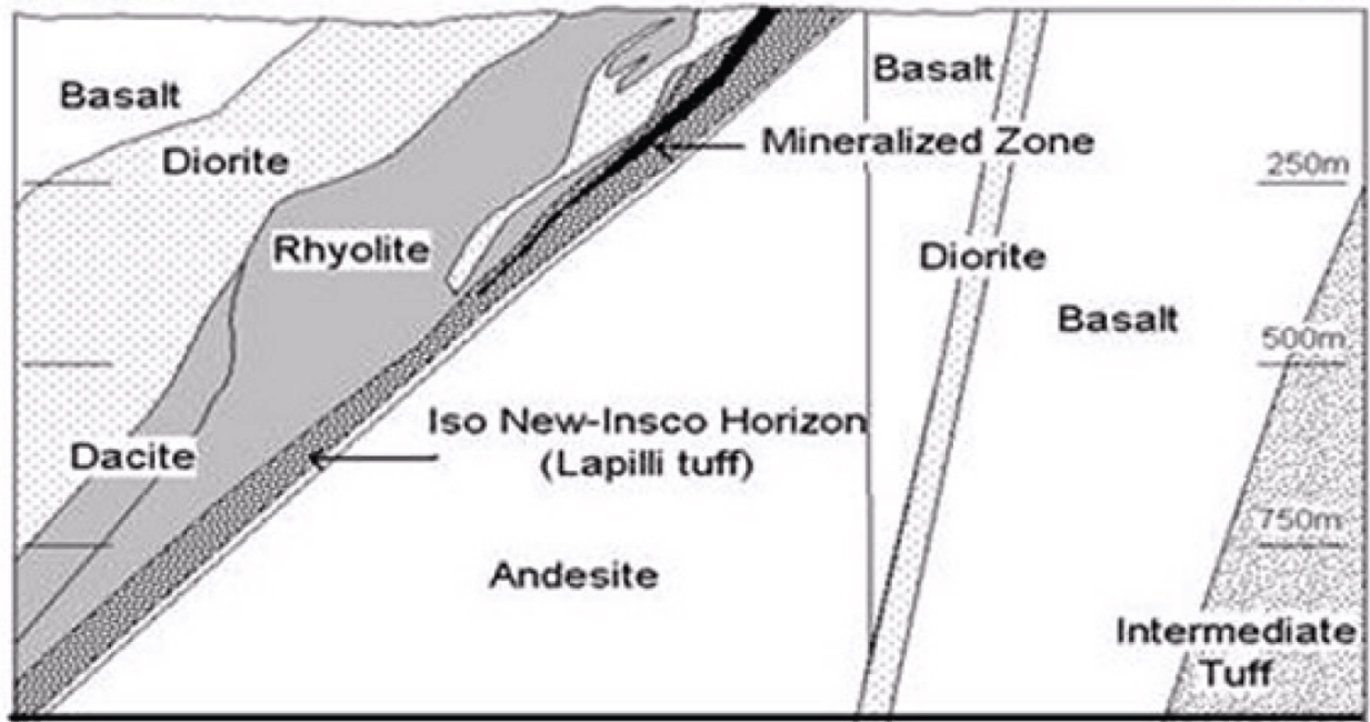
Figure 7.8 Simplified geological cross section of the Magusi deposit looking west where the Iso New-Inasco Horizon represents the favourable horizon which is also the host to the Fabie Bay deposit. Note the stratigraphy is overturned. (2005, Cheng et.al.)
