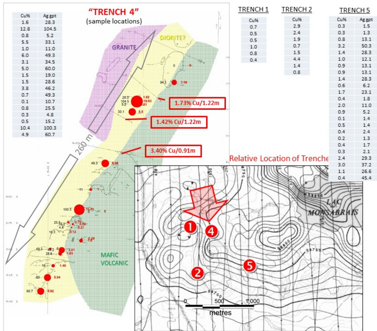
Figure 7.17 Moose Lake target historic trenching (Trench 4) and sampling summary. This is a historic illustration with geology extracted from historic assessment files. (1959, Nealon Mines; 1988, Aunore and Aunorex) Inset of total field magnetic contour map also extracted from historic files showing relative location of historic trenches. A summary of grab sample results for all four trenched areas, circa 1959 and 1988 is included. Compiled December 2021 from Québec Government SIGEOM web site assessment files. Due to the nature of the
