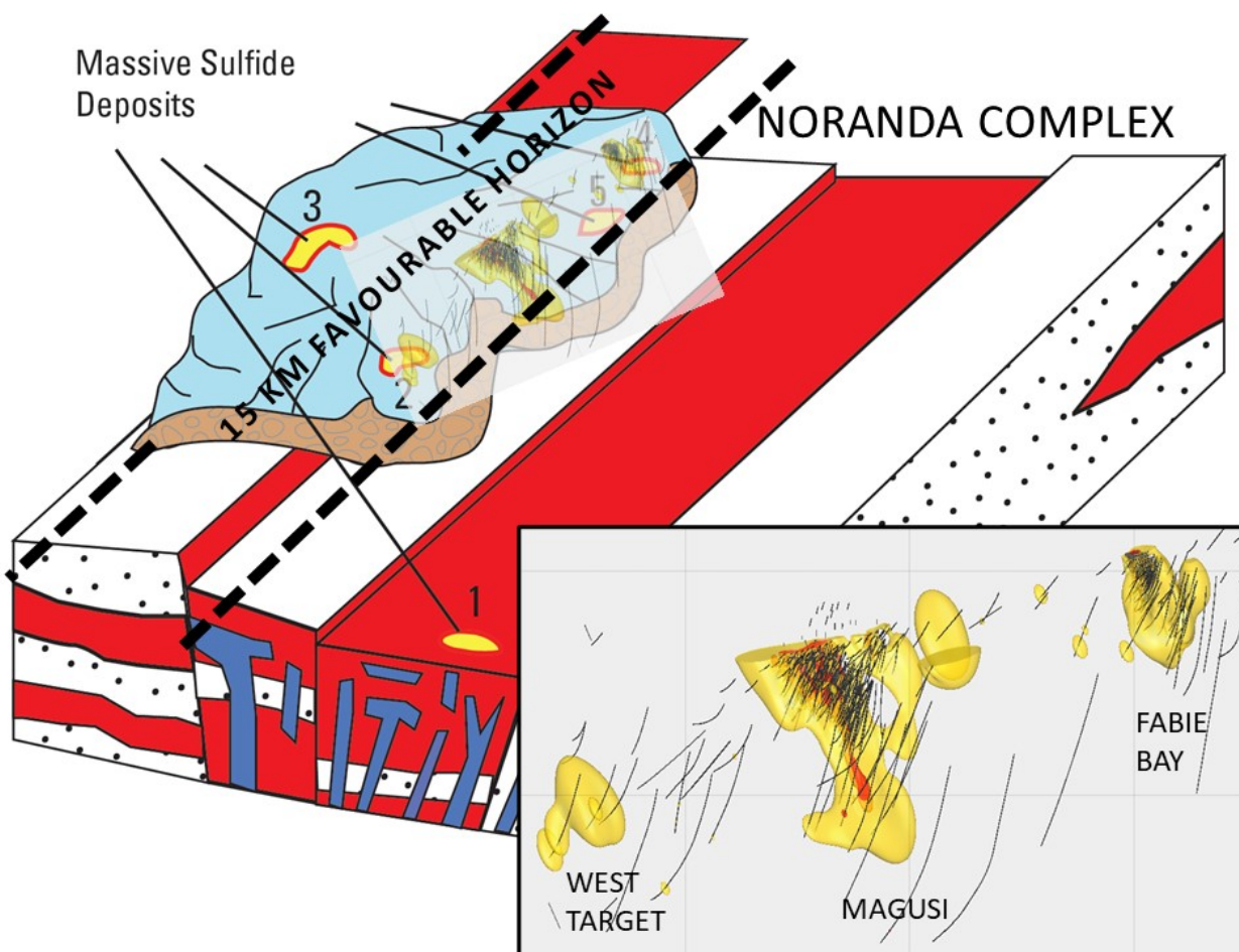
Figure 25.1 Schematic representation of the geological setting of the project area and relative location of the favourable horizon and current Magusi and Fabie Bay deposits, looking northeast, and initial target areas. Location 1 potential targets A and B, 2 represent the interpreted geological setting for the West or East target, location 3 the Moose Lake area, location 4 the Fabie Bay deposit, and location 5 the lenses along the favourable horizon in this model. After 2012, Morgan and Klaus.
