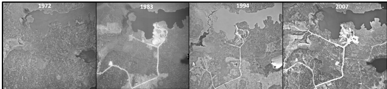
Figure 6.8 Sequence of four air photo showing the development of the project area prior to the initial development of the Fabie Bay deposit until the restart of mining activities in 2007. Each air photo is approximately 15 km wide. North is to the top of the air photos. (2007, National Air Photo Library, Natural Resources Canada in Ottawa)
