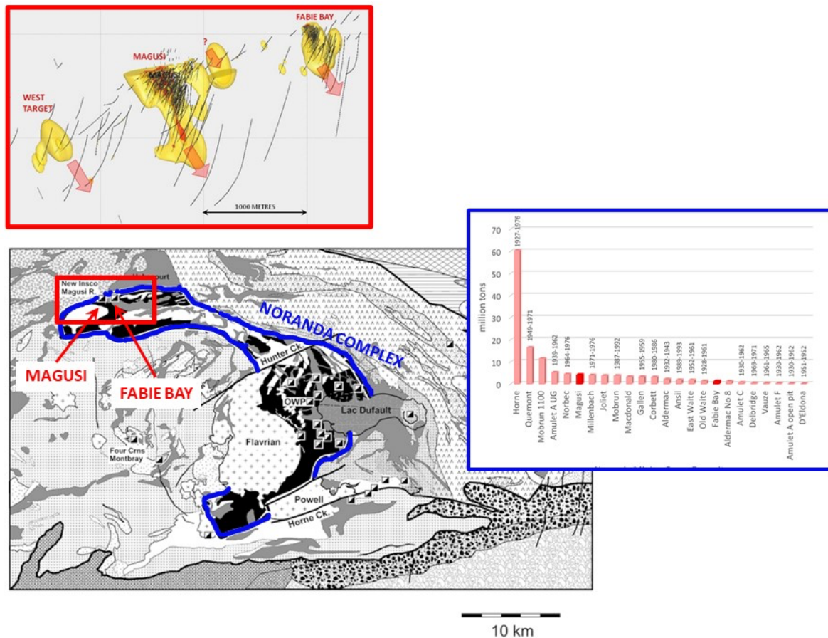
Figure 1.2 Location of project area in NW corner of the Noranda Complex, host to the Noranda Mining Camp of VMS deposits. See Figures 6.1, 6.2, 7.2 for details. Compiled March, 2022, North to the top of diagram.
