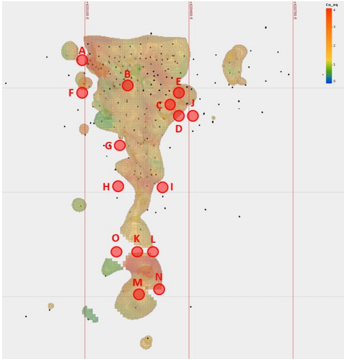
Figure 7.13 Longitudinal section historic interpretive (based on the RPA (2012) estimate) sketch of the Magusi deposit looking north, showing the Cu equivalent grade and conceptual Phase One drilling (Holes A through M) and conceptually contingent Phase Two drill holes (N&O). The sketch illustrated the relative intensity of mineralization. Cu equivalent cutoff grade of 0.5% applied to the model. Compiled by Electro Metals, March 2022. Metal prices and estimates of recoveries as follows: Copper $3.26/lb 80%, zinc $1.24 per pound 72%, gold $1626 per oz 60%, silver $20.71 per oz 40% - prices are three – year look back prices as at March 2022, recoveries are conservative estimates as agreed with management for potential payable recoveries. Cu-eq calculation: [(\text{Cu Grade} \times \text{Cu Price} \times \text{Cu Rec}) + (\text{Zn grade} \times \text{Zn Price} \times \text{Zn Rec}) + (\text{Ag Grade} \times \text{Ag Price} \times \text{Ag Rec}) + (\text{Au grade} \times \text{Au Price} \times \text{Au Rec})] / \text{Cu Price} / 22.046 , where Rec = potential recovery estimated to the best of management's and Author's knowledge. Magusi deposit dips south at approximately 50°.
