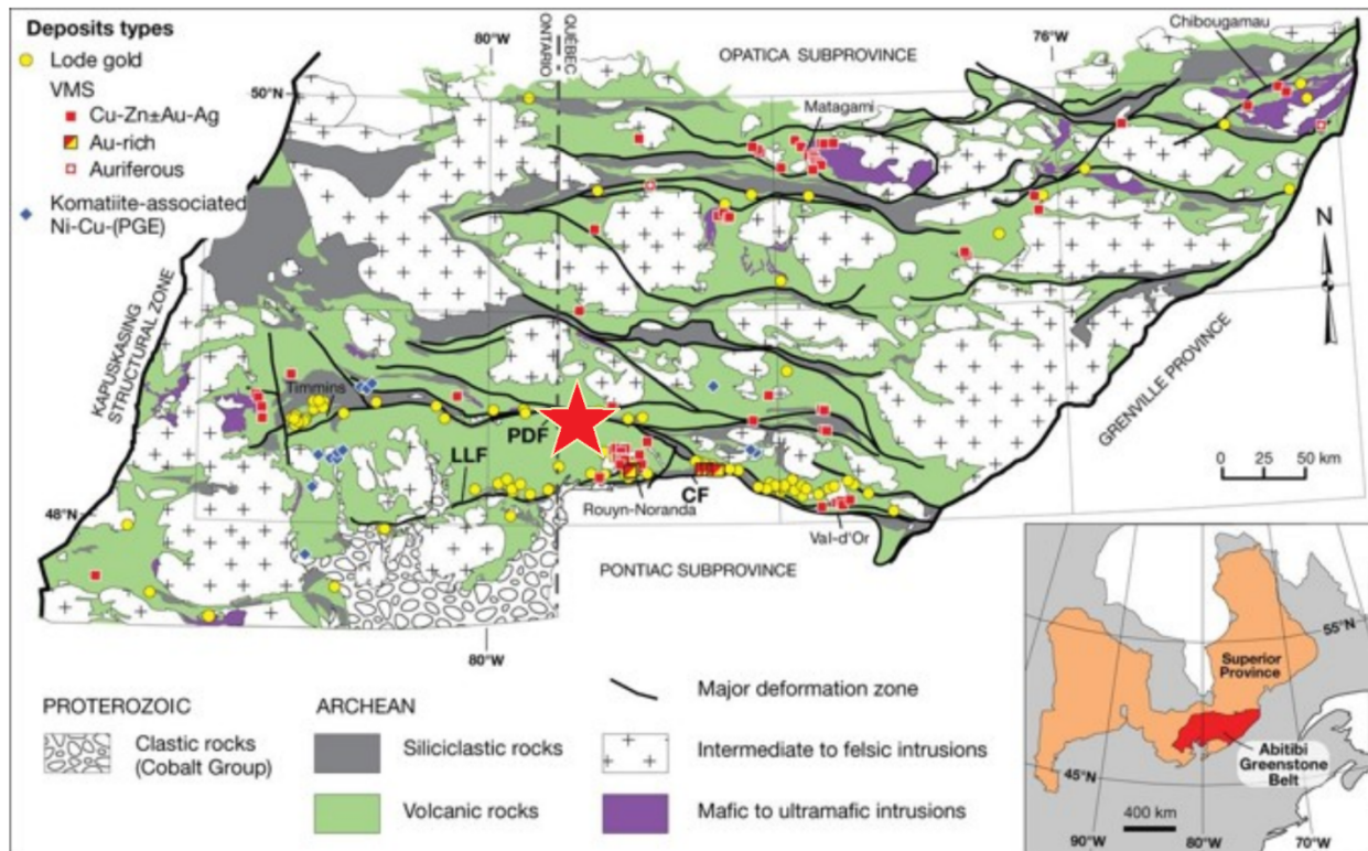
Figure 7.1 Location of major greenstone-hosted deposits in the Abitibi greenstone belt. CF and LLF=Larder Lake-Cadillac deformation, PDF= Porcupine-Destor deformation zone. (2014, Mercier-Langevin et al.) Project area shown as RED STAR.
