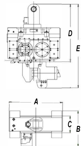
Dimension Layout Of Vibratory Driver/Extractor
