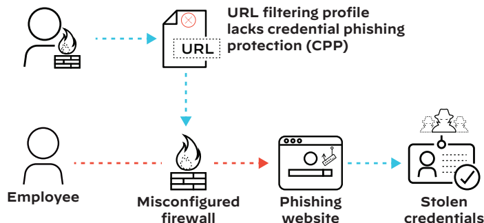
Figure 8: Without credential phishing prevention, hackers can steal credentials and exfiltrate data
