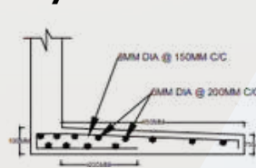
Typical Cross Section of RCC Chejja
