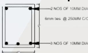
Typical Cross Section of RCC Chejja
